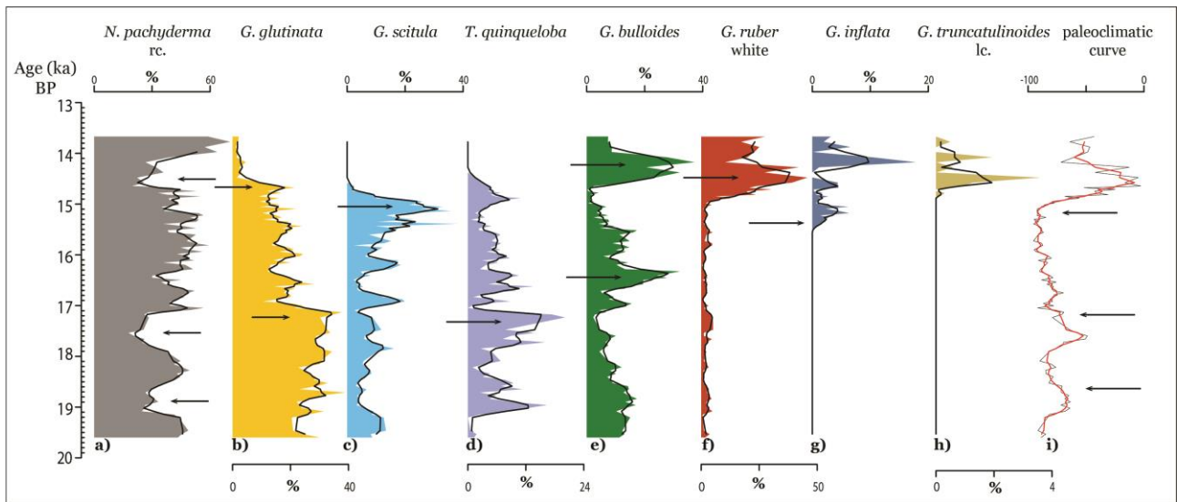
267 268 Fig. 4: Foraminifera assemblage relative abundance from core ND14Q-AR2 (%; thick line 3-points average), 269 and foram-based paleoclimate curve (thick line 3 points average). Black arrows indicate significant 270 increases/decreases in abundances as signalled in the text.
