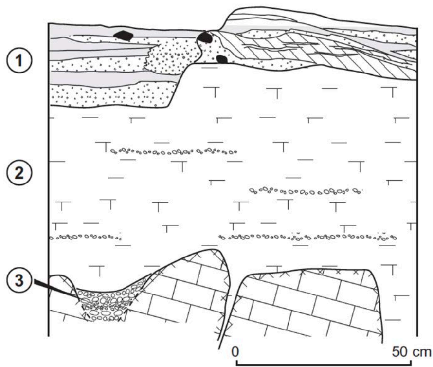
Figure 4 : Stratigraphy of the deposits in the lower chamber of the Cave of the Monk observed on the east section of the first test pit. The numbers indicate the stratified units.
