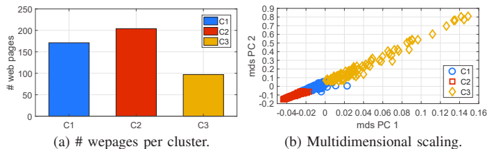
Fig. 5: Obtained web page clusters with K = 3 -means.
