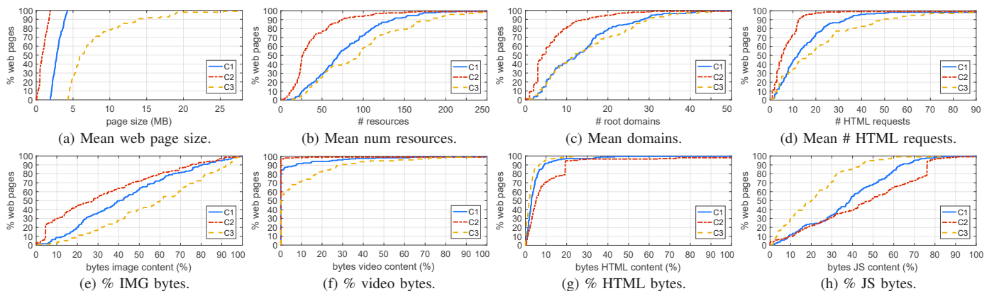
Fig. 6: Characterization of web pages per cluster. Web page size is a clear differentiator for cluster membership.
