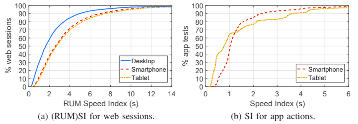
Fig. 5: (RUM)SI for web sessions and app actions.
