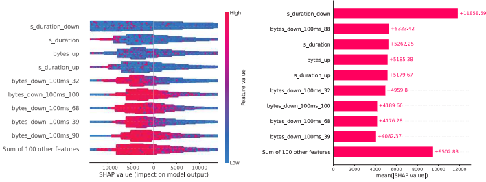
(a) SHAP-value distributions. (b) Mean absolute SHAP-values. Fig. 9: Explainability of DeepQoE , for web browsing and apps.
