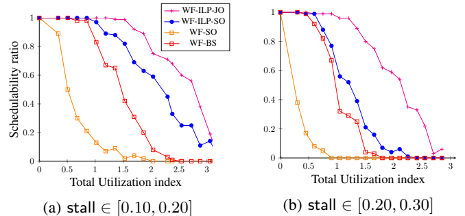
Fig. 3: Schedulability of ILP vs heuristics approaches
