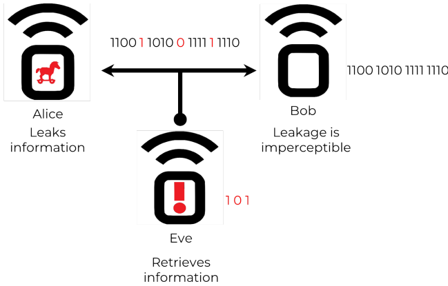
Fig. 1. Threat model.
