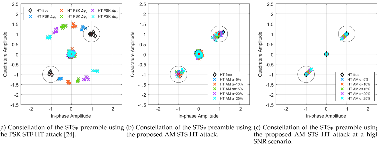
Fig. 15. Measurement results from the STS constellation test.
