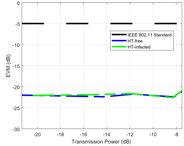
Fig. 12. Measured EVM of the transmitted BPSK signal from an AM STS HT-infected device and an HT-free device, along with the IEEE 802.11 standard EVM specification [36].
