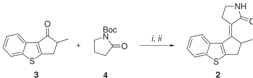
Fig. 5 | Synthesis of MTDP. Reagents and conditions: (i) LiHMDS, \text{BF}_3 \cdot \text{Et}_2\text{O} , THF dry, -78^\circ\text{C} ; (ii) TFA, DCM, 0^\circ\text{C} to room temperature.
