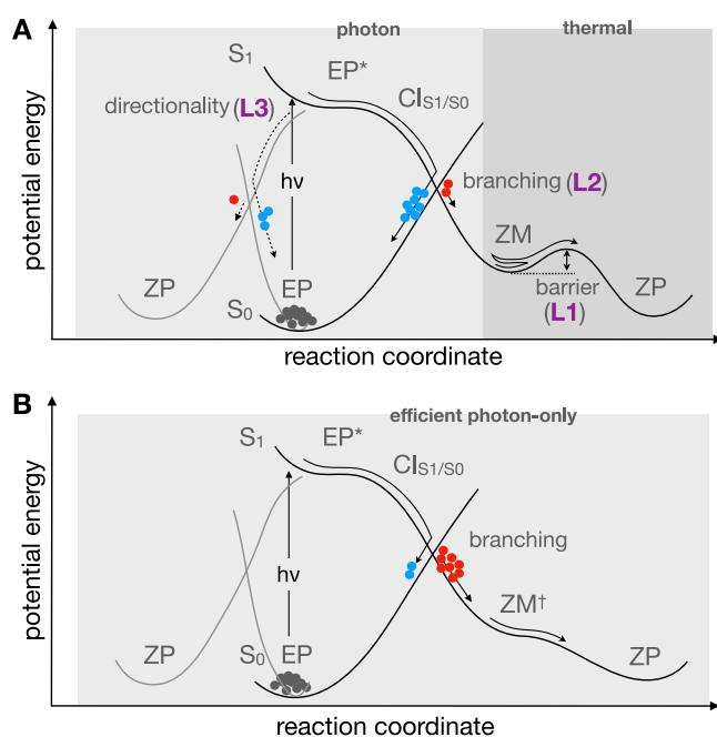
Fig. 2 | Schematic representation of the reaction path for the first half of LDRM working cycle starting from an EP configuration. A Classic unidirectional EP \xrightarrow{h\nu} ZM \rightarrow ZP half-cycle with the possibility of loss of EP \xrightarrow{h\nu} ZP directionality. The labels marking the system potential limitations (see text) are given in purple. B Target unidirectional, efficient, and ultrafast EP \xrightarrow{h\nu} ZP half-cycle. The acronyms EP, ZP, etc. stand for the structures with a specific helicity (P or M) in a specific configuration (Z or E). CI stands for conical intersection. The gray dots represent the initial structures, the red dots represent the productive trajectories, and the blue dots the unproductive trajectories.
