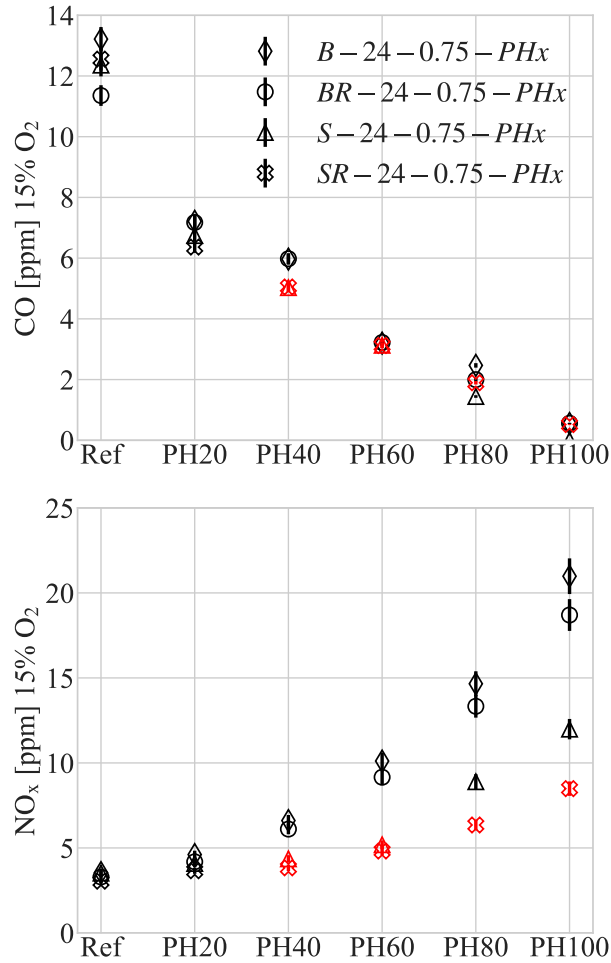
Fig. 8. CO and NO x emissions with error bars as a function of the hydrogen content for different DFDS burner geometries Geo - 24 - 0.75 - PHx . Black symbols: Anchored flames. Red symbols: Lifted flames.
