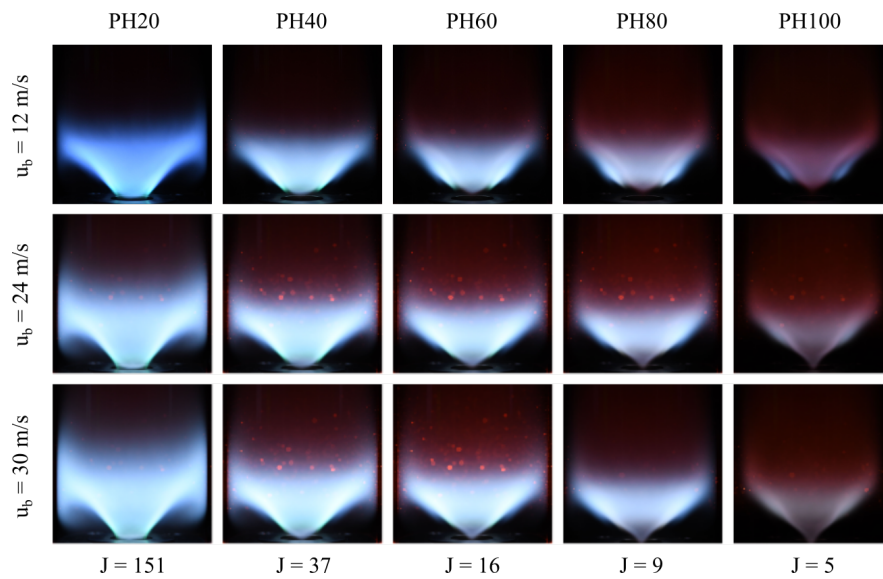
Fig. 2. Effect of air bul velocity on flame stabilisation for SR - u_{e0} - 0.75 - PHx . Images are recorded in the visible spectrum.
