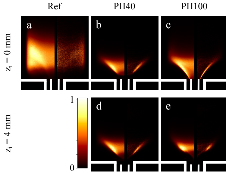
Fig. 7. \text{OH}^* intensity distribution collected in the line of sight (images on the left) and after Abel deconvolution (images on the right) for B - 24 - 0.75 - PH_x (top row) and SR - 24 - 0.75 - PH_x (bottom row).
