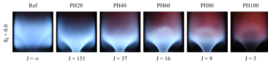
Fig. 1. Effect of the injector recess on flame stabilisation for BR - 24 - 0.75 - PHx . Images are recorded in the visible spectrum.
