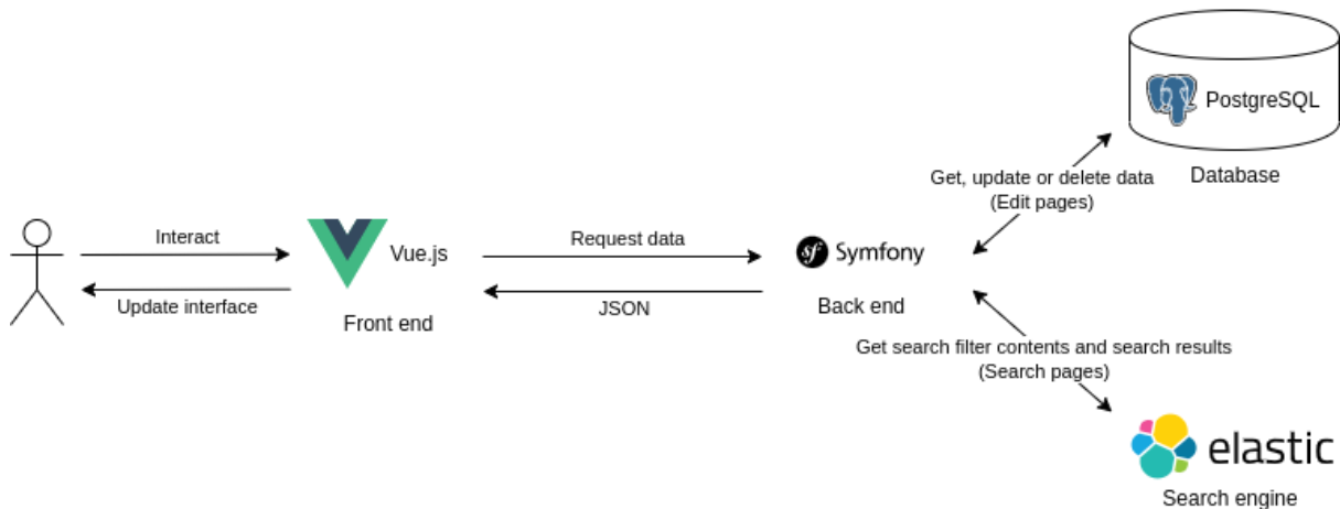
Figure 17: Overall architecture of the current version of the online platform (interactions after the initial page load on edit and search pages)
