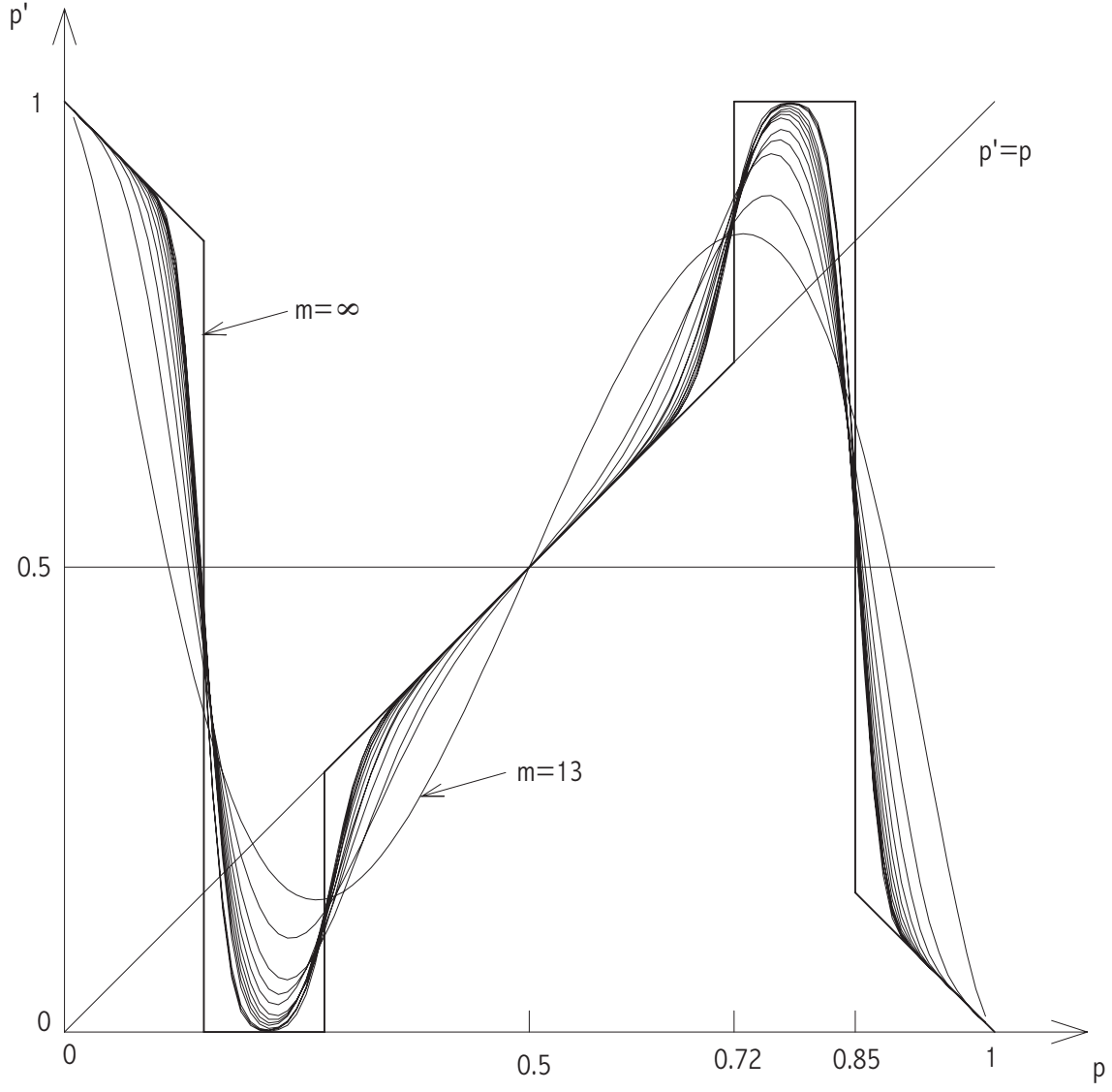
Figure 1: The family of functions F_{\underline{\rho},m}(p) for \rho_{hb} = \rho_{bh} = 0.72 and \rho_{hh} = \rho_{bb} = 0.85 . The curves are for m = 13 + j \cdot 26, j = 0, \dots, 13 . Note the convergence to the function G_{\underline{\rho}} , (indicated by m = \infty ).
