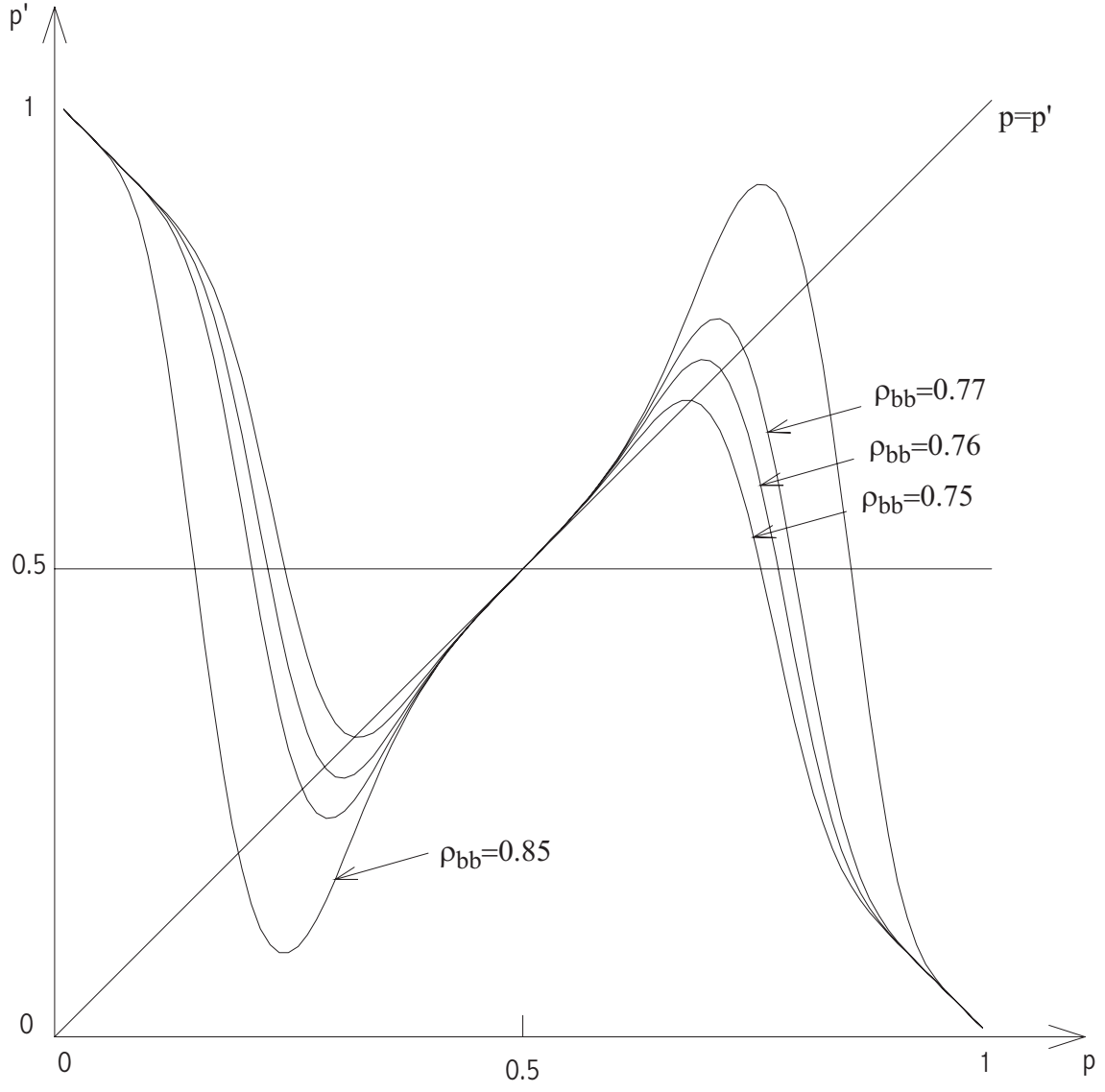
Figure 2: Four curves F_{\rho,m} , for m = 60 and \rho_{hh} = \rho_{bh} = 0.72 , with \rho_{hh} = \rho_{bb} = 0.75, 0.76, 0.77, 0.85 .
