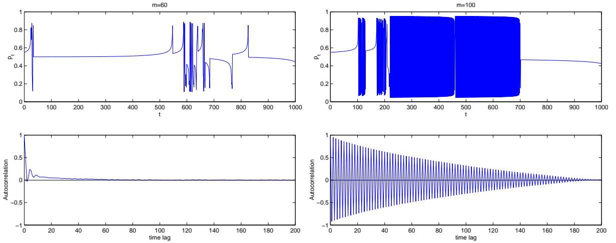
Figure 11: The upper panels represent the time series p_t for m = 60 (left) and m = 100 (right). The lower panels represents the corresponding autocorrelation function of r_t \propto p - 1/2 for m = 60 (left) and m = 100 (right) with the same parameters \rho_{hb} = \rho_{bh} = 0.72 and \rho_{hh} = \rho_{bb} = 0.85 .
