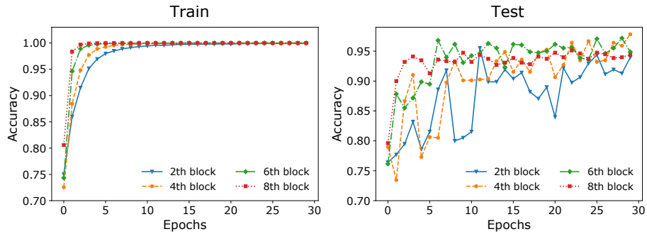
Fig. 3. Convergence of the models
