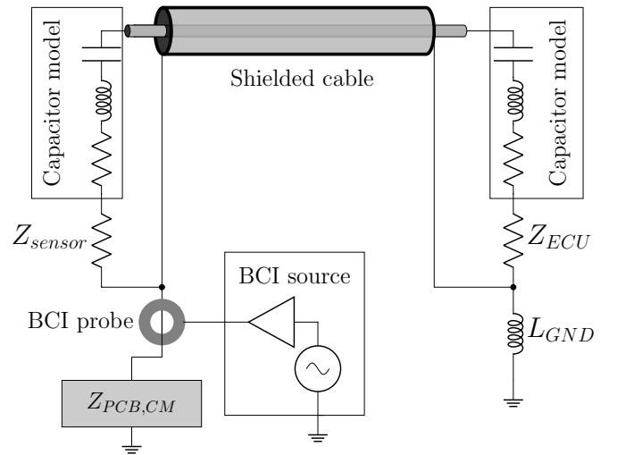
Fig. 5. BCI test simulation schematic
