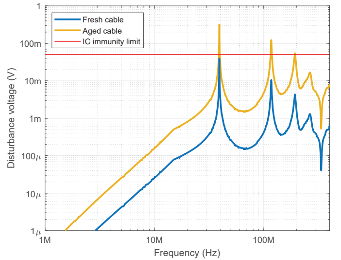
Fig. 7. BCI test simulation results at ECU IC input pin
