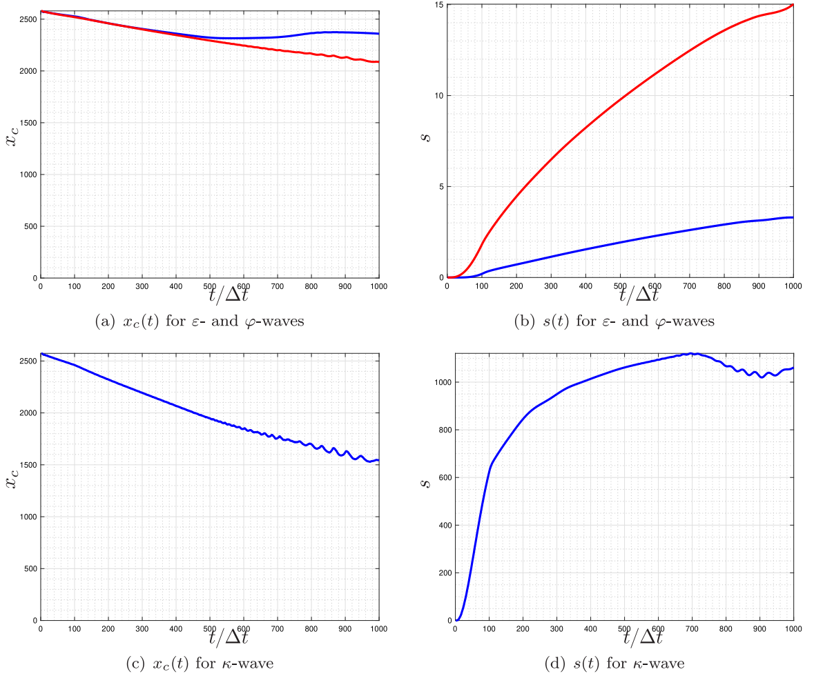
Fig. 10. Evolution of the centroid x_c and of the variance s for \varepsilon -, \varphi - and \kappa -waves in the case of the rectangular impulse with \bar{p} = 1000 N and t_i = 0.005 s. In the plots (a) and (b), blue and red colors refer to \varepsilon -, \varphi -waves, respectively. (For interpretation of the references to color in this figure legend, the reader is referred to the web version of this article.)
