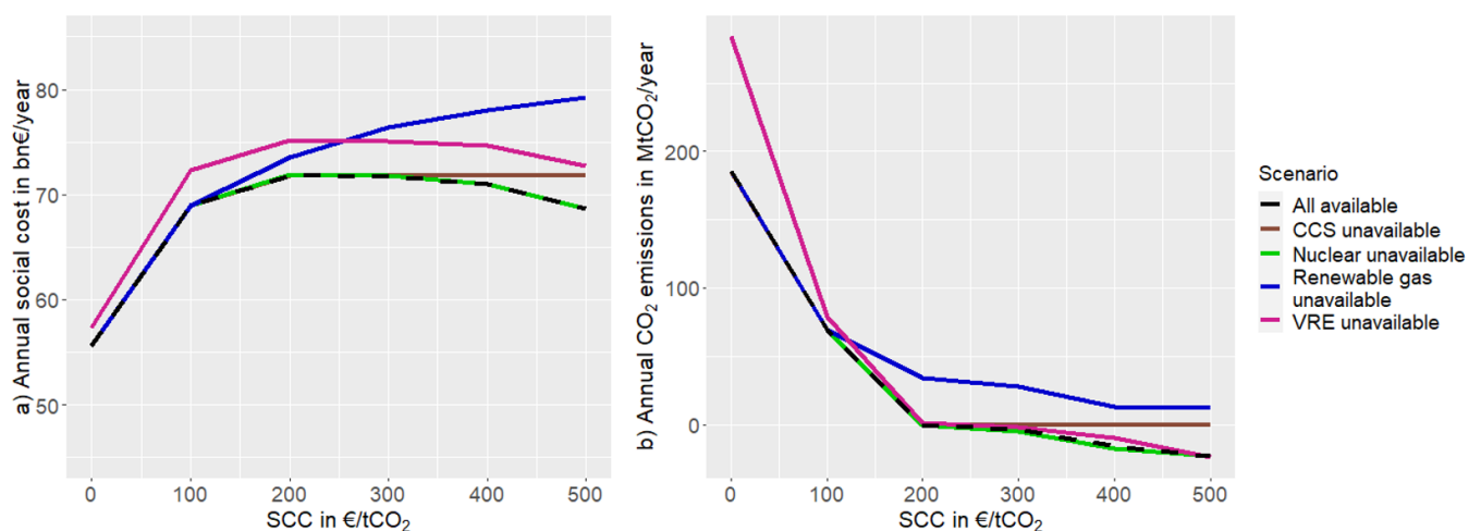
Figure 10. a) Annual social cost and b) annual CO 2 emissions of the energy systems for different technology availability scenarios
