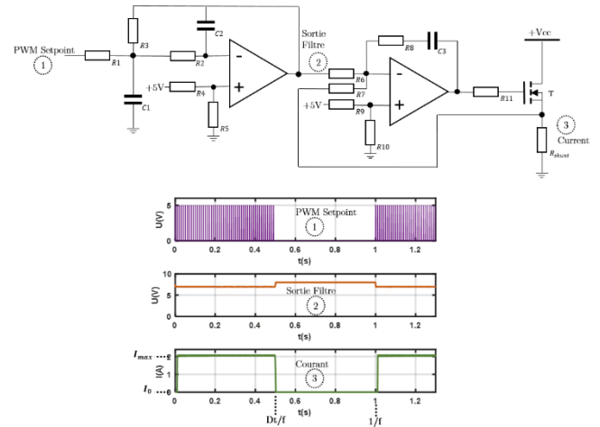
Figure 12. Analog control of drain current
