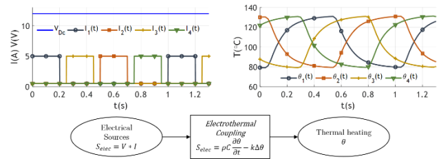
Figure 4. 1Hz cycling simulation example (*)
