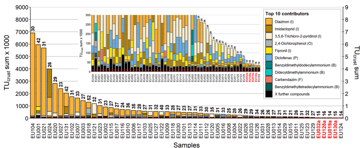
Fig. 12. Risk driving compounds according to TU_{\text{crust}}\text{sum} (based on dataset B; NA = MDL/2 ). The bars represent TU_{\text{crust}}\text{sum} for each sample. The coloured stacks within the bars represent the compound-specific TUs of the top 10 contributors by maximum TU (over all samples), and are sorted by increasing values. Further compounds are aggregated in the black coloured stacks at the bottom of each bar (“X further compounds”). The bold line indicates the risk threshold of 1. The dashed line indicates the risk threshold incl. a dilution factor of 10. Samples from WWTPs with advanced treatment are highlighted in red (suffix “a”). (For interpretation of the references to colour in this figure legend, the reader is referred to the web version of this article.)
