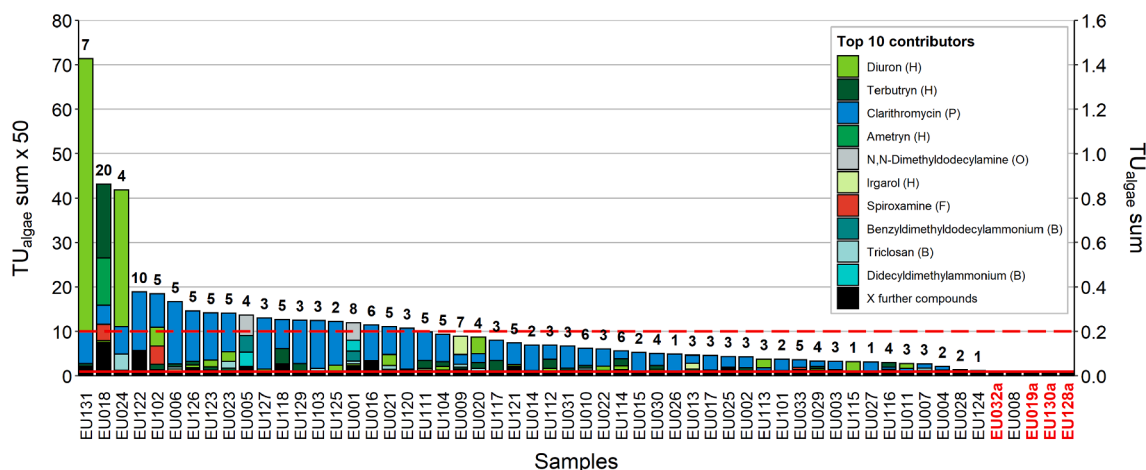
Fig. 11. Risk driving compounds according to TU_{\text{algae}}\text{sum} (based on dataset B; NA = MDL/2 ). The bars represent TU_{\text{algae}}\text{sum} for each sample. The coloured stacks within the bars represent the compound-specific TUs of the top 10 contributors by maximum TU (over all samples), and are sorted by increasing values. Further compounds are aggregated in the black coloured stacks at the bottom of each bar (“X further compounds”). The bold line indicates the risk threshold of 1. The dashed line indicates the risk threshold incl. a dilution factor of 10. Samples from WWTPs with advanced treatment are highlighted in red (suffix “a”). (For interpretation of the references to colour in this figure legend, the reader is referred to the web version of this article.)
