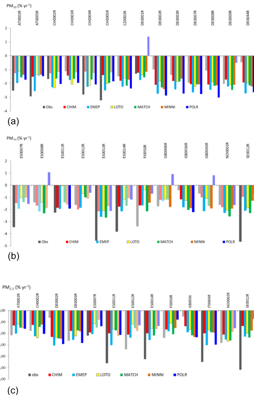
Figure A8. Mean observed (black) and modelled (coloured) relative trends for \text{PM}_{10} (a, b) and \text{PM}_{2.5} (c) in the period 2000–2010 at the individual trend sites. Insignificant modelled trends are shown as striped bars. Units: \% \text{ yr}^{-1} .
