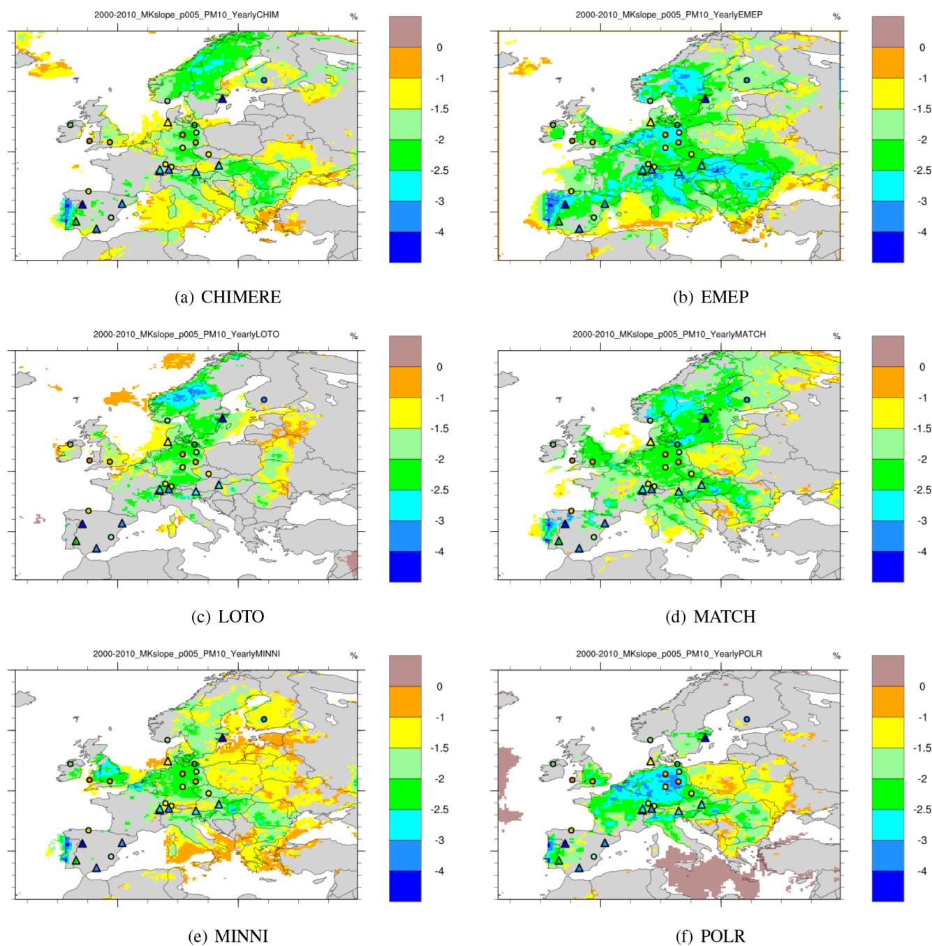
Figure A5. Mean Sen slopes relative to the starting year of 2000 (% yr -1 ) for PM 10 trends in the period 2000–2010 calculated by the individual models. The modelled trends are shown as a coloured contour map (grey or white means non-significant trends) and the observed trends as coloured triangles (significant) and circles (non-significant).
