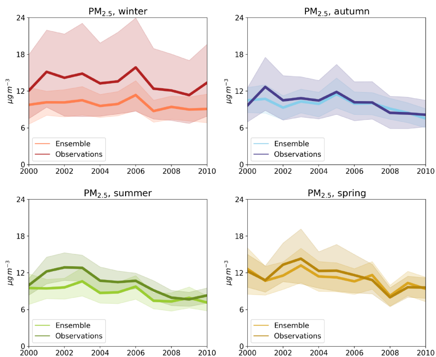
(b) \text{PM}_{2.5}
