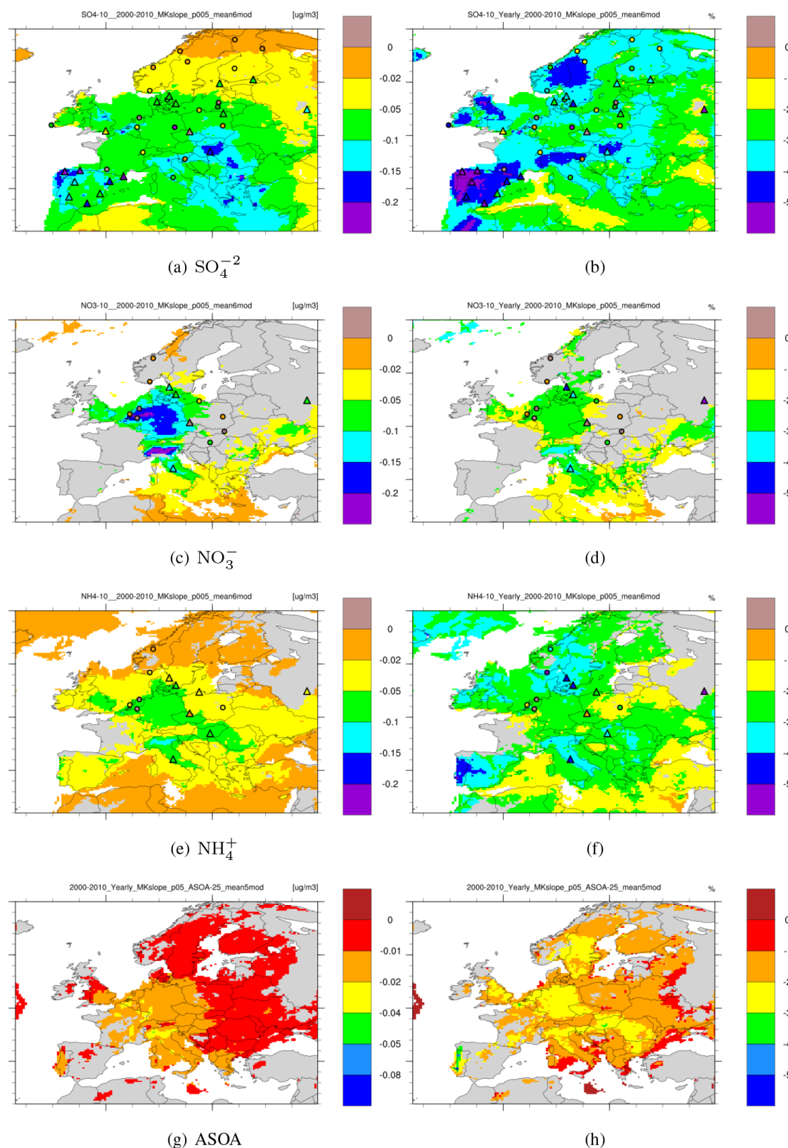
Figure A9. Mean Sen trend slopes, observed and from six-model ensemble, for 2000–2010 for anthropogenic aerosols \text{SO}_4^{-2} , \text{NO}_3^- and \text{NH}_4^+ (a–f) and simulated with the five-model ensemble for ASOA (note the different colour scale). (a, c, e, g) Absolute ( \mu\text{g m}^{-3} \text{yr}^{-1} ) and (b, d, f, h) panels – relative ( \% \text{yr}^{-1} ) trends. The modelled trends are shown as the coloured contour map (grey or white means non-significant trends) and the observed trends as coloured triangles (significant) and circles (non-significant).
