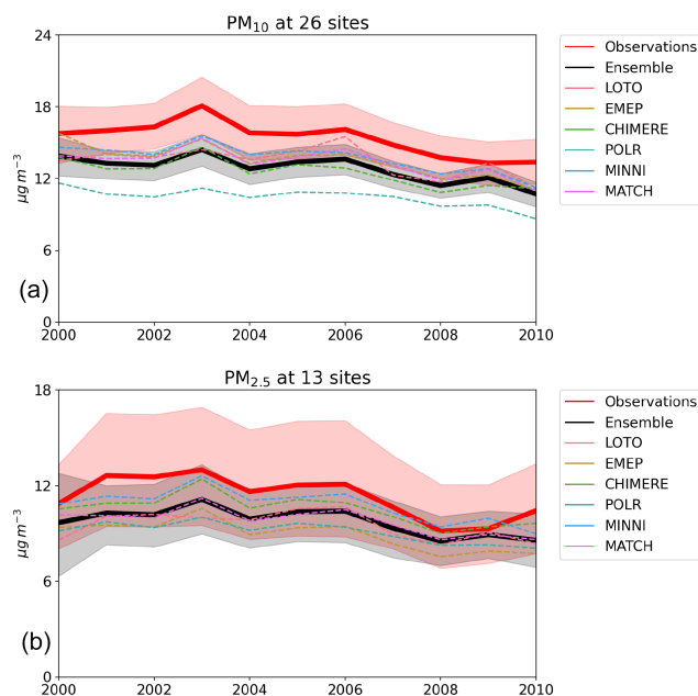
Figure 4. Observed and simulated with the six-model ensemble and the individual models' annual mean concentrations of \text{PM}_{10} (a) and \text{PM}_{2.5} (b) for the period 2000–2010, averaged over the trend sites. The 95 % confidence intervals for observed and ensemble modelled PM concentrations are shown with shaded areas. The number of sites with available observations for the individual years can be found in Table 1. (Note: \text{PM}_{10} from POLR does not include coarse sea salt; see the text for explanations.)
