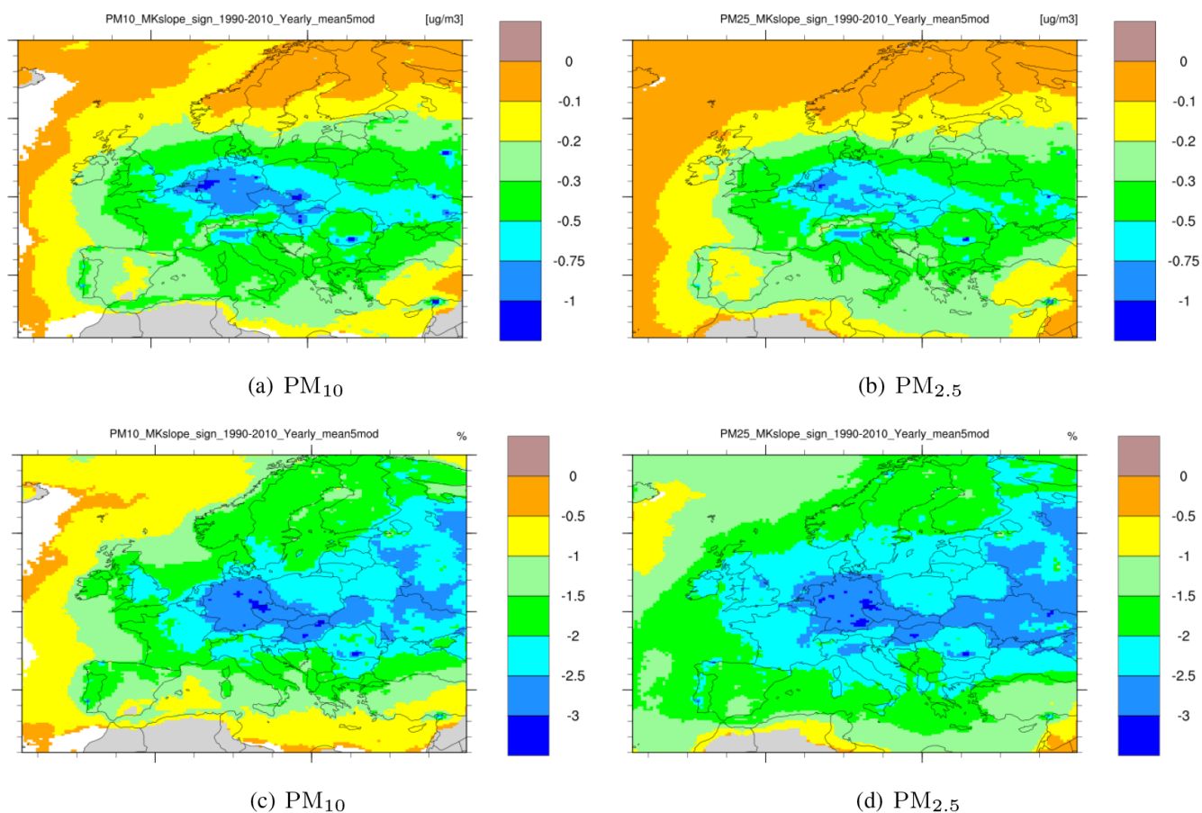
Figure A13. Annual mean Sen slope for trends in the period 1990–2010 as calculated by the six-model ensemble ( a , c ) for \text{PM}_{10} and ( b , d ) \text{PM}_{2.5} . Upper panels – absolute ( \mu\text{g m}^{-3} \text{ yr}^{-1} ) – and lower panels – relative to 1990 ( \% \text{ yr}^{-1} ).
