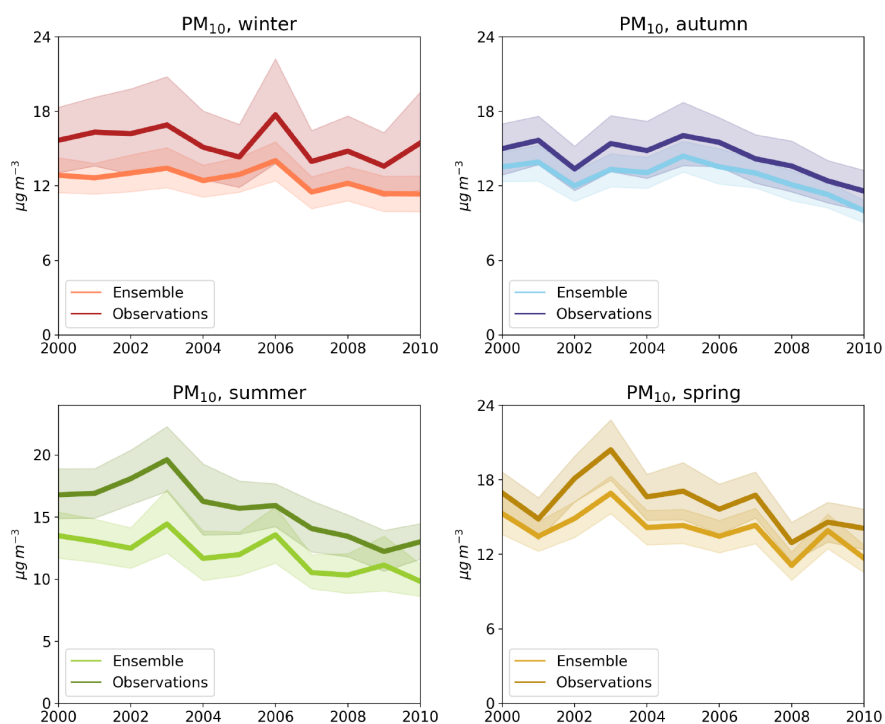
(a) \text{PM}_{10}
