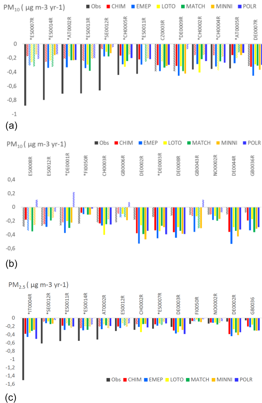
Figure A7. Observed and modelled trend slopes ( \mu\text{g m}^{-3} \text{yr}^{-1} ) for the period 2000–2010 at the trend sites for PM 10 (a, b) and for PM 2.5 (c). The sites are sorted by decreasing observed negative trends; insignificant trends are shown as striped bars. Units: \mu\text{g m}^{-3} \text{yr}^{-1} .
