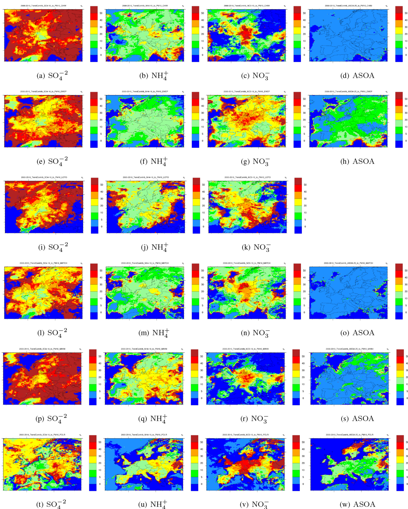
Figure A11. Relative contributions of (from left to right) \text{SO}_4^{2-} , \text{NH}_4^+ , \text{NO}_3^- and ASOA to PM 10 trends between 2000 and 2010 calculated by (from top to bottom) the CHIMERE, EMEP, LOTOS-EUROS, MATCH, MINNI and Polair3D models.
