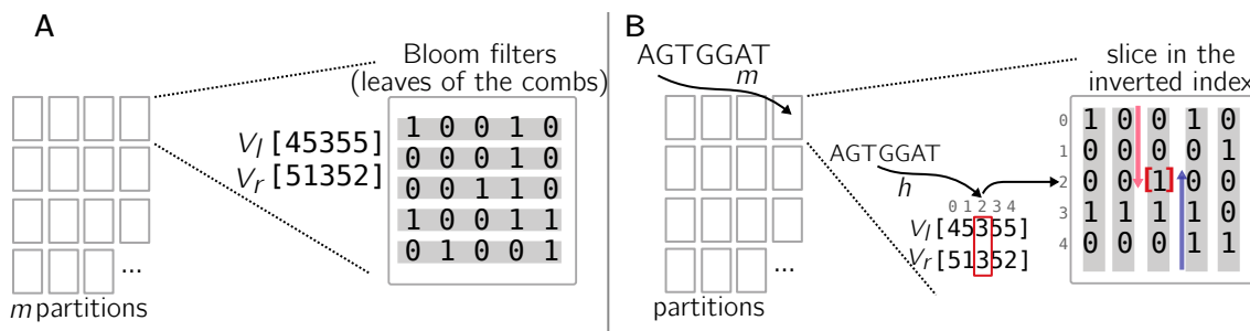
Figure 4: Panel A: the content of one partition in PAC. The aggregative Bloom comb trees constructed for a given partition are represented using leaves BF's (in grey) and two aggregative BF's V_l and V_r . Panel B: a single query in the same partition as Panel A. The index has been inverted. A k -mer enters a PAC by finding the partition corresponding to its minimizer. V_l and V_r are loaded, and a search space (here [3] only) is defined given the position obtained by hashing the k -mer (here the k -mer's hash value is 2). Then, a slice is extracted from the inverted index at the given position, and bits are checked to find 1's. Here there's a single position, so necessarily an 1.
