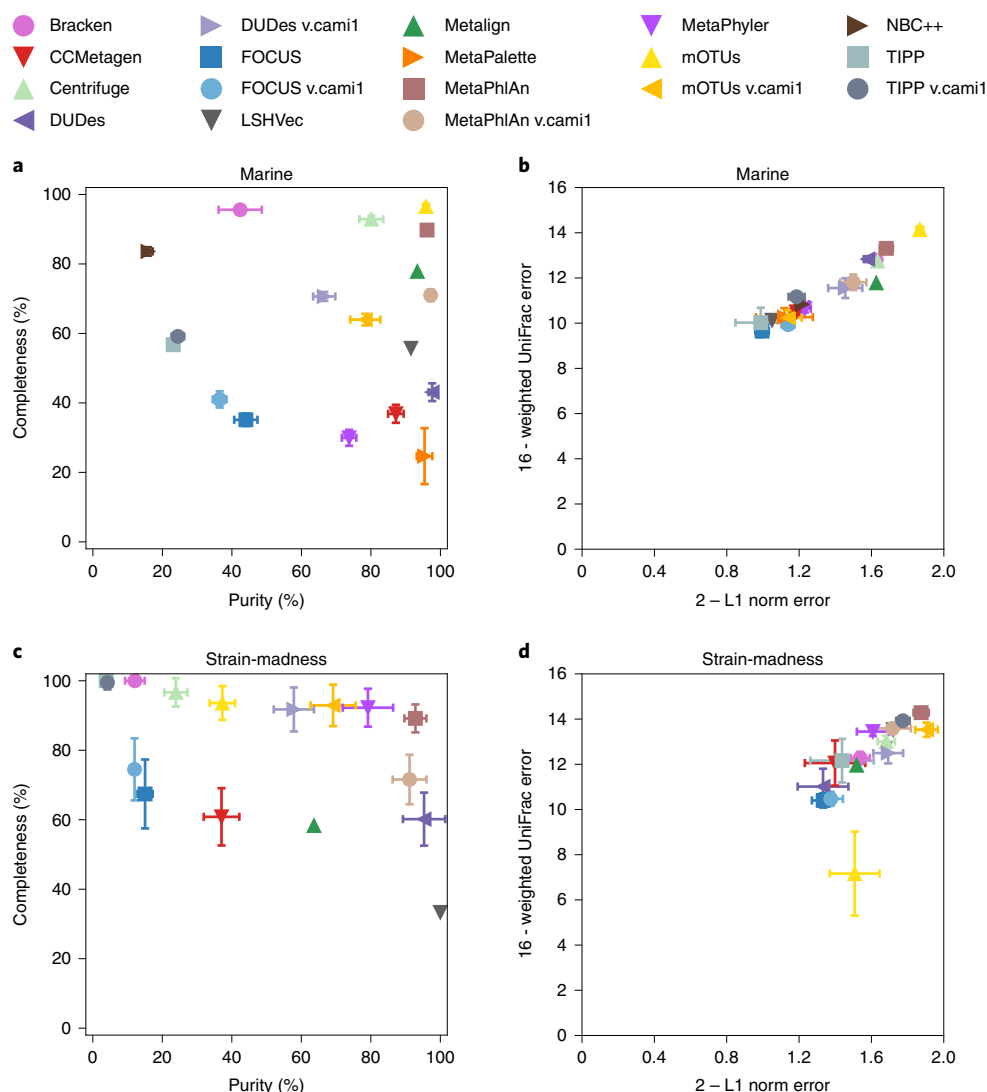
Fig. 4 | Taxonomic profiling results for the marine and strain-madness datasets at genus level. a,b, Marine datasets. c,d, Strain-madness datasets. Results are shown for the overall best ranked submission per software version (Supplementary Tables 33 and 35, and Supplementary Fig. 12). a,c, Purity versus completeness. b,d, Upper bound of L1 norm (2) minus actual L1 norm versus upper bound of weighted UniFrac error (16) minus actual weighted UniFrac error. Symbols indicate the mean over ten marine and 100 strain-madness samples, respectively, and error bars the standard deviation. Metrics were determined using OPAL with default settings.
