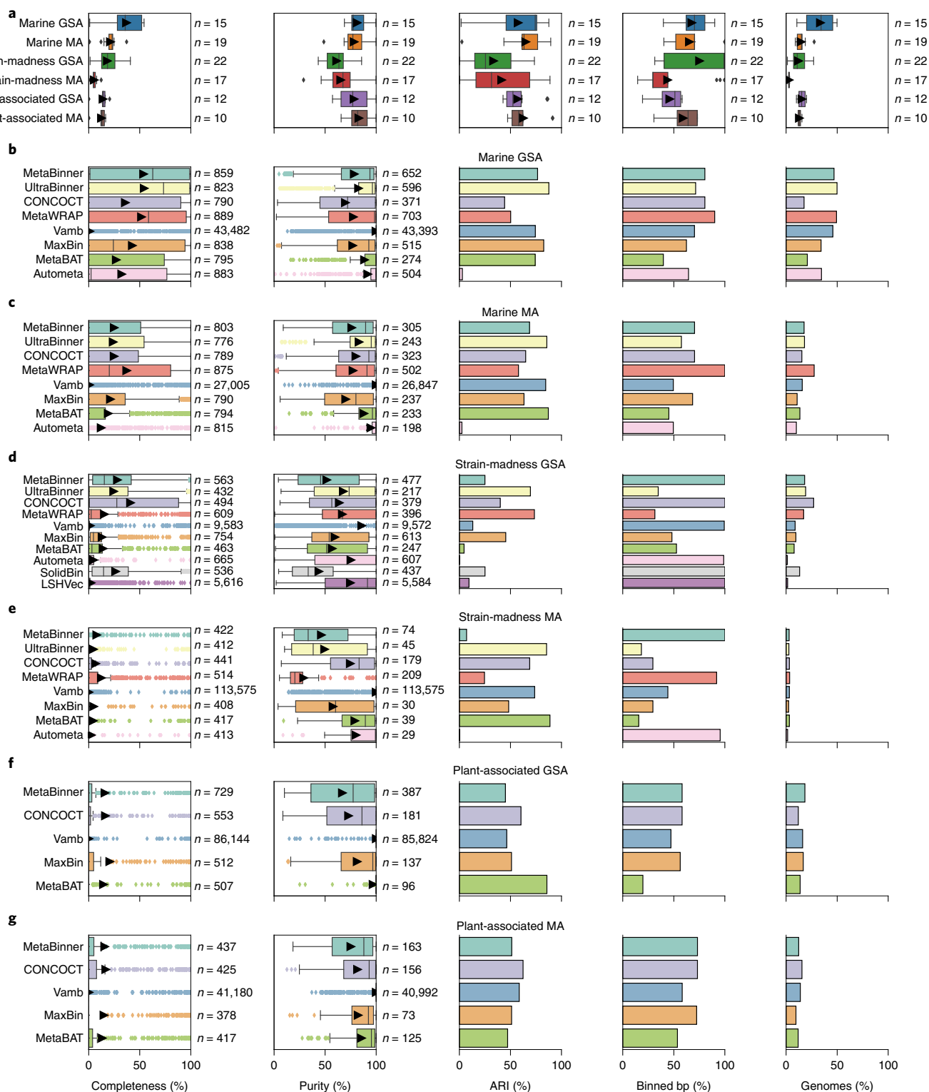
Fig. 2 | Performance of genome binners on short-read assemblies (GSA and MA, MEGAHIT) of the marine, strain-madness, and plant-associated data. a , Boxplots of average completeness, purity, ARI, percentage of binned bp and fraction of genomes recovered with moderate or higher quality (>50% completeness, <10% contamination) across methods from each dataset (Methods). Arrows indicate the average. b–g , Boxplots of completeness per genome and purity per bin, and bar charts of ARI, binned bp and moderate or higher quality genomes recovered, by method, for each dataset: marine GSA ( b ), marine MA ( c ), strain-madness GSA ( d ), strain-madness MA ( e ), plant-associated GSA ( f ) and plant-associated MA ( g ). The submission with the highest F1-score per method on a dataset is shown (Supplementary Tables 9–15). Boxes in boxplots indicate the interquartile range of n results, the center line the median and arrows the average. Whiskers extend to 1.5 × interquartile range or to the maximum and minimum if there is no outlier. Outliers are results represented as points outside 1.5 × interquartile range above the upper quartile and below the lower quartile.
