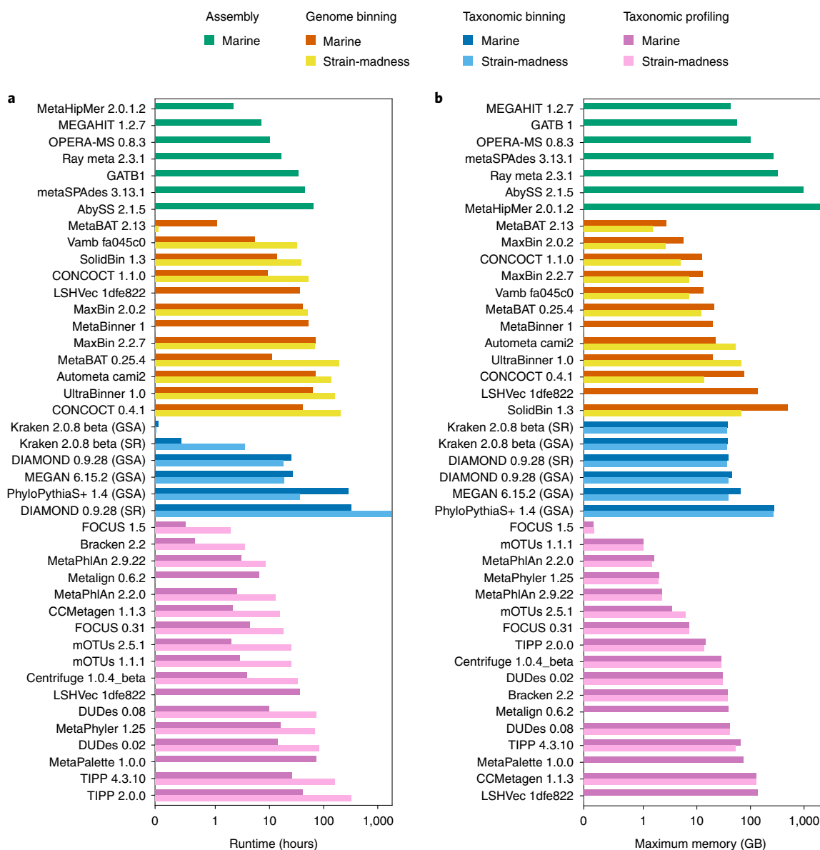
Fig. 5 | Computational requirements of software from all categories. a, Runtime. b, Maximum memory usage. Results are reported for the marine and strain-madness read data or GSAs (Supplementary Table 40). The x axes are log scaled and the numbers given are the software version numbers.
