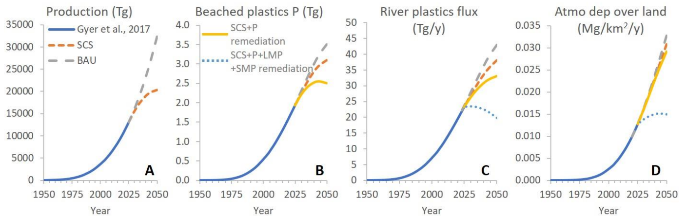
Figure 4. Box model results for plastics cycling from 1950 to 2050. From 1950 to 2015 the model estimates the dispersal of P, LMP and SMP in different Earth surface reservoirs, based on known plastics production and waste generation. From 2015 to 2050 the model illustrates plastics production (A), amount of beached macroplastics, P (B), the total, P+LMP+SMP, annual river plastics flux (C), and atmospheric deposition (atmo dep) to remote land surfaces (D), for two different scenarios with different plastics production and waste disposal trajectories: business as usual (BAU, grey dashed line) (3), and systems change scenario (SCS, orange short dashed line) (4), the latter representing feasible plastics policy implementation. Despite the large difference in plastics production towards 2050, 991 vs 168 Tg y -1 in BAU and SCS, environmental stocks and fluxes recover only slowly due to the large mobilization of mismanaged plastics from the terrestrial discarded plastics pool that continue to cycle between land, ocean and atmosphere. Two remediation scenarios are simulated for the 2025 to 2050 period: Discarded P remediation at a rate of 3% per year (yellow solid line), and combined discarded P, LMP and SMP remediation at a rate of 3% per year. See Methods and SI for details on BAU and SCS.
