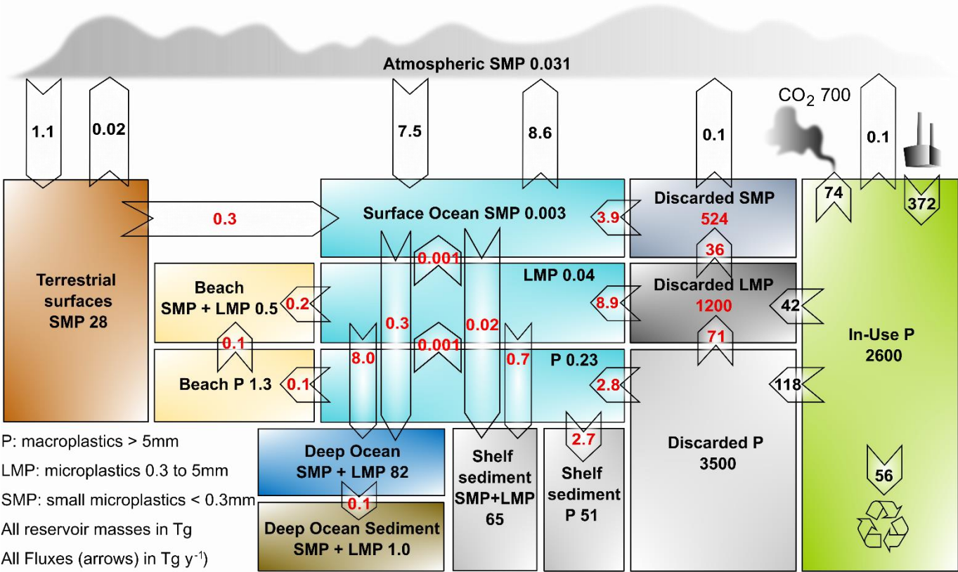
Figure 1. Global plastics budget and cycle for the year 2015. Reservoir sizes are shown in teragrams (Tg), and fluxes in Tg y -1 (arrows). Three plastics size classes are considered: macroplastics > 5mm (P), microplastics from 0.3 to 5mm (LMP), and small microplastics <0.3mm (SMP) that can become airborne. The discarded (Disc) plastic pools represent the terrestrial technosphere, including urban-industrial areas, landfills, agricultural soils impacted by mulching or waste disposal, wetlands, and other impacted ecosystems. The remote terrestrial reservoir lies outside the technosphere and is only impacted by airborne SMP deposition, re-emission and runoff. Numbers in black are based on observations, and numbers in red on box model optimization. Uncertainties are provided in Table 4.
