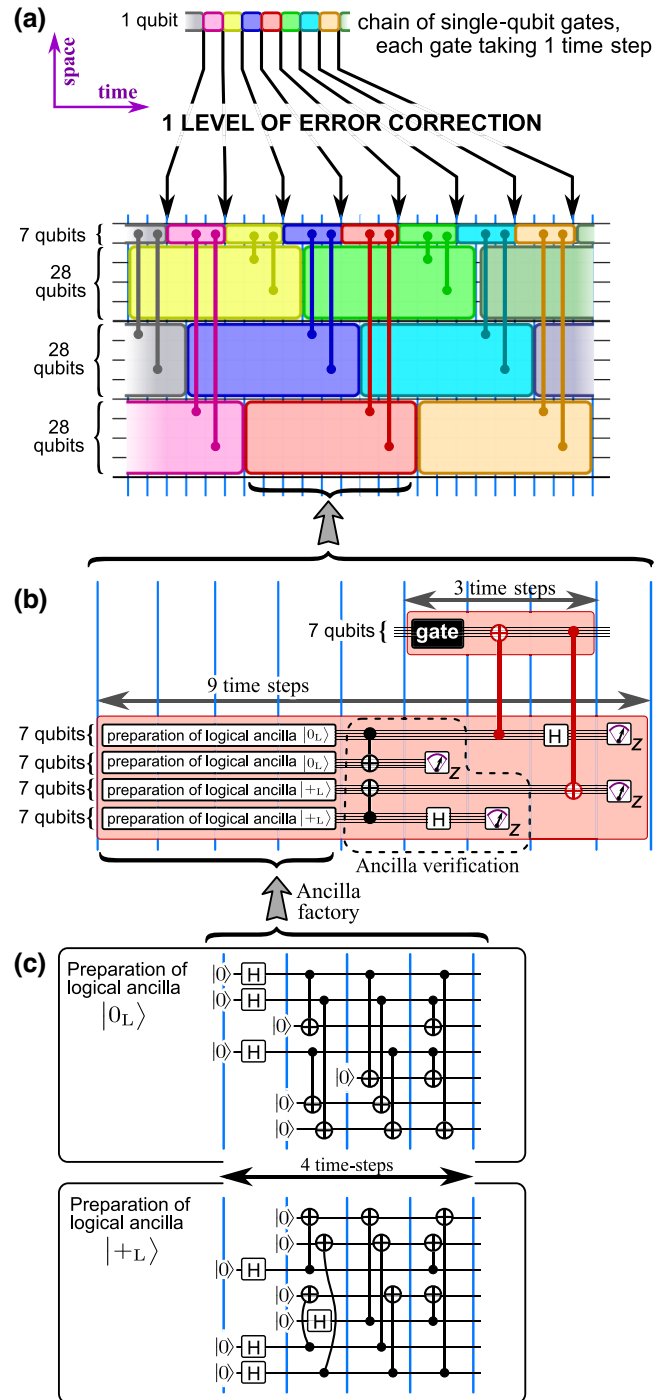
FIG. 8. The circuit for one level of the seven-qubit error-correction code on a series of single-qubit gates [89,90]. Gates acting on groups of seven qubits are transversal. The ancilla factory prepares the state of the logical ancillas [92]. The vertical blue lines indicate time steps in the algorithm. See the main text for a brief description of this circuit, with additional technical details given in Appendix A.
