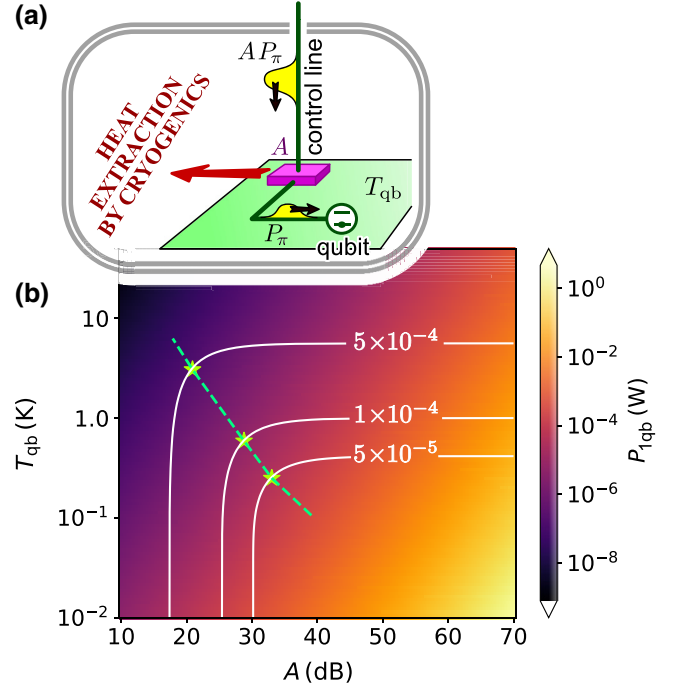
FIG. 2. (a) A sketch of our simplified model of a single qubit in a cryostat. (b) The color scale is the power consumption (in watts) of a single-qubit gate as a function of the qubit temperature T_{\text{qb}} and attenuation A . The parameter values are \gamma^{-1} = 1 ms and \tau_{1\text{qb}} = 25 ns. Each contour is associated with the target metric (worst-case infidelity) indicated in white. The green stars mark the optimal parameters (those that minimize the power consumption) for each value of the target metric.
