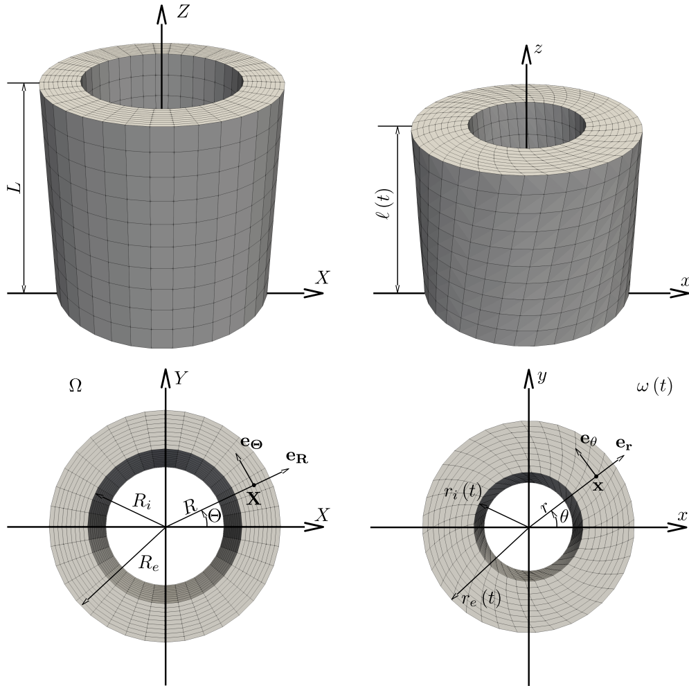
FIGURE 1 Geometry and kinematics of the cylindrical model. Note that the cylinder is actually closed (see Figure 2), but the lids are not represented here.
