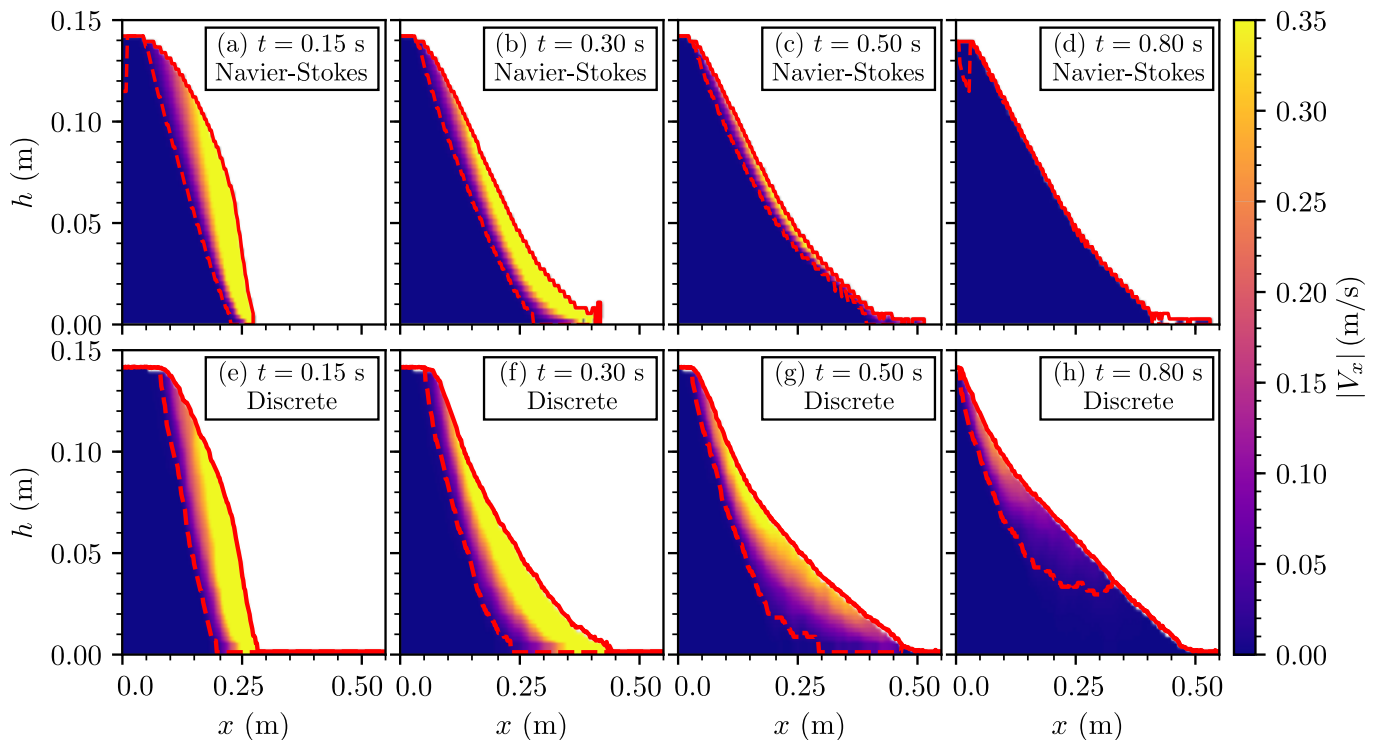
FIG. 4. Comparison between the horizontal velocity V_x calculated with the Navier-Stokes (Basilisk) (first row) and discrete (COCD) (second row) simulations, for \theta = 0^\circ . The red continuous line represents the free surface while the red dashed line the static/flowing transition, considering a threshold value V_x = 1 \text{ cm s}^{-1} , as in [17]. Figures (a,e) belong to the acceleration phase, (b,f), to the deceleration phase and (c,d,g,h) to the stopping phase.
