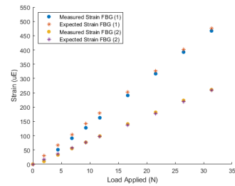
Figure 4: Measured vs Expected Strain on Defective Beam
