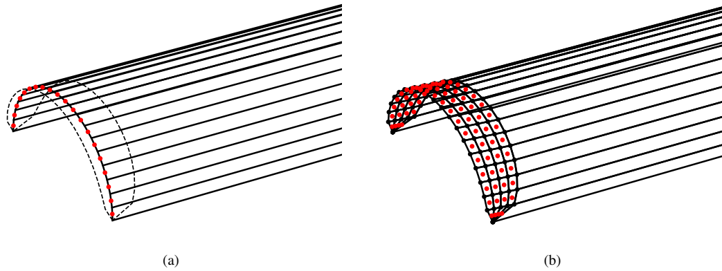
Figure 1: Vortex assemblies for the lifting line (a) and lifting surface (b) methods. The red dots represent the control point.
