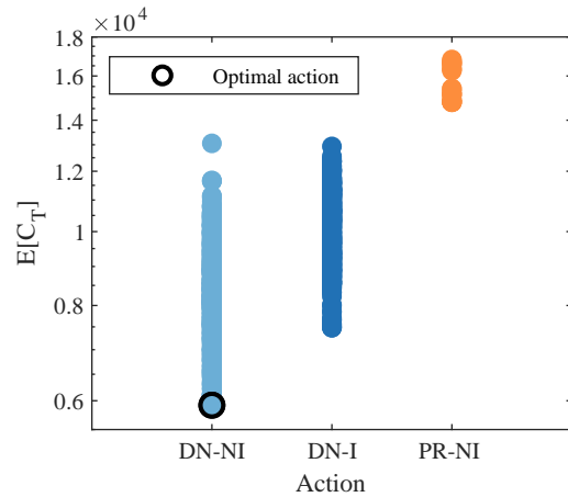
(b) Expected total cost associated with each \alpha -vector (and corresponding action).
