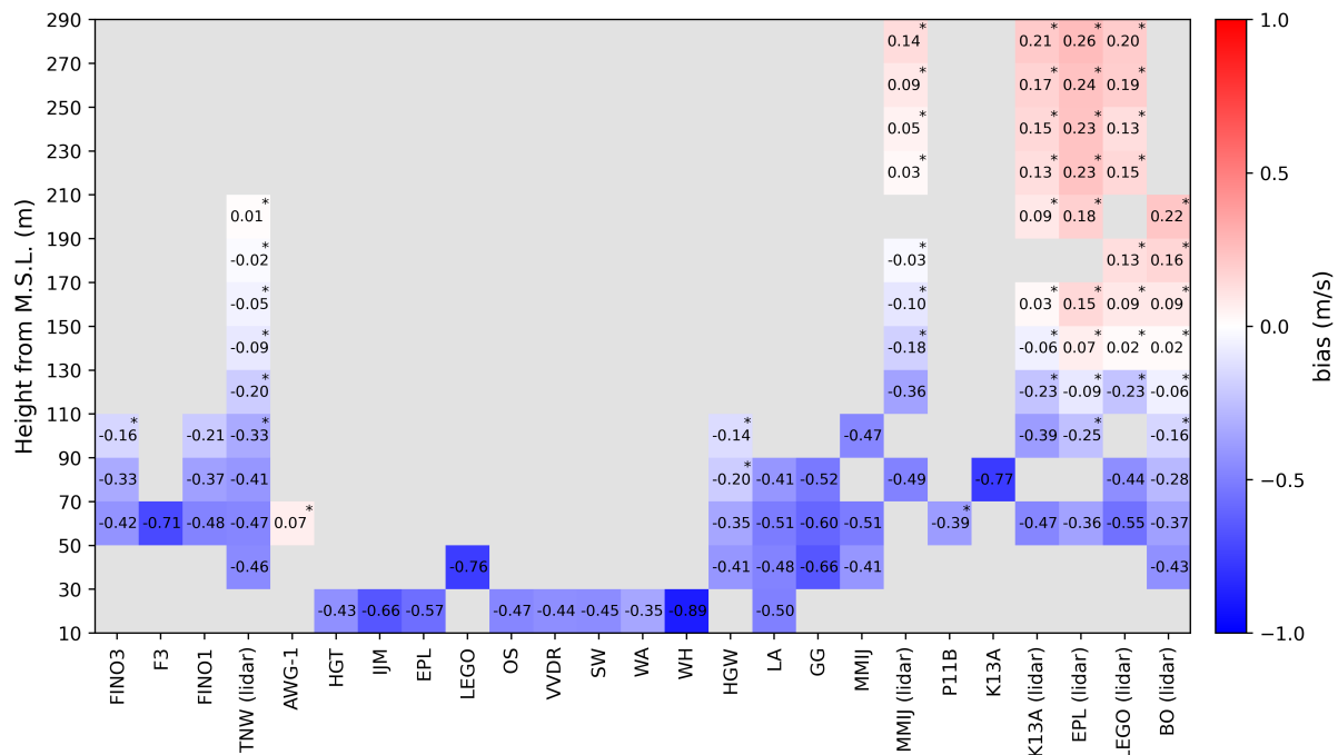
Figure 2: Wind speed bias (m/s) for the complete time period of the measurement data. This concerns measurements between 10 and 290 meters to MSL. The vertical range is subdivided into 20 meter intervals for readability. Stations are clustered per region.
