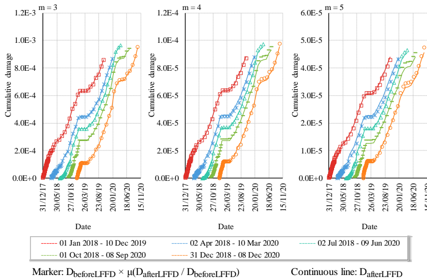
Figure 3. Accumulated damage calculated using LFFD recovery – continuous lines – versus accumulated damage without LFFD recovery scaled by the average damage ratio ( \mu ) (average of damage ratios after 300 days) – markers –.
