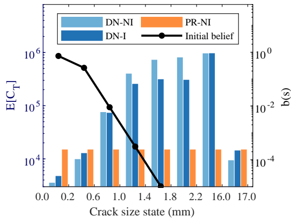
(a) Initial belief (black line) and state values of three \alpha -vectors (colored bars).
