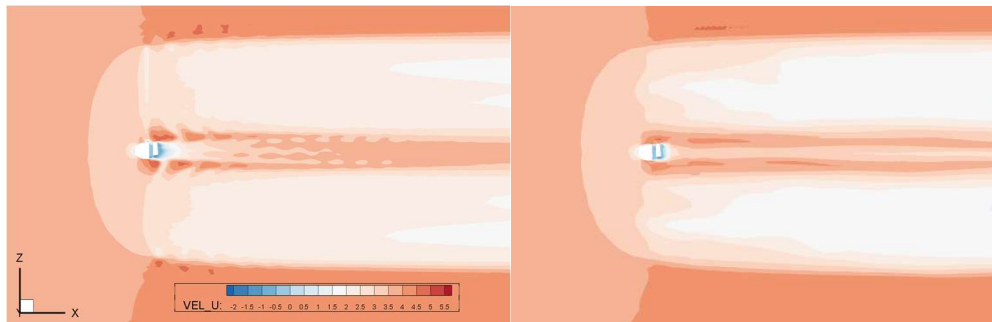
Figure 2 Axial velocity contour, comparisons between ALM (left) and RADM (right)
