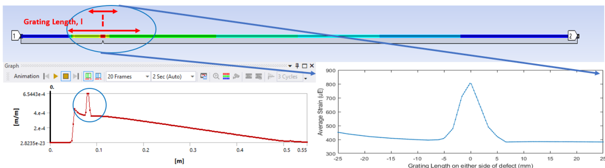
Figure 8: FEA for Defective Beam with Different FBG sensing lengths
