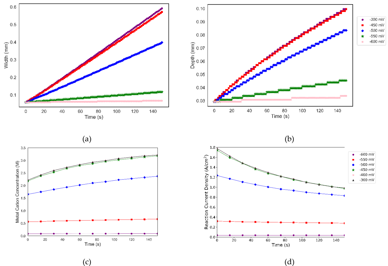
Figure 2: For a range of applied potentials: evolution of (a) pit width vs. time. (b) pit depth vs. time. (c) metal cation concentration vs. time. (d) reaction current density vs. time.
