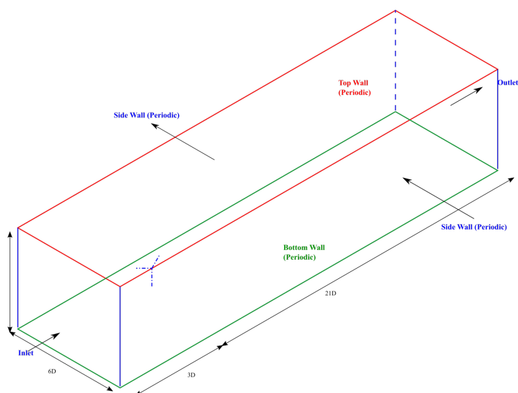
Figure 1: Flow Domain
