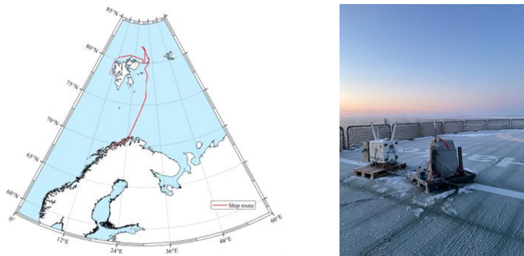
Figure 1- Path of cruise during the campaign (left), the dotted lines indicate the periods when systems were not operating. Lidars positioning and setup on board R/V Kronprins Haakon (right).
