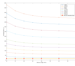
Figure 7: Average Strain estimated for different FBG sensing lengths
