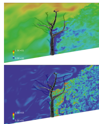
(d) IBM simulation for major model tree structures; instantaneous velocity (top) and vorticity (bottom) [20].
