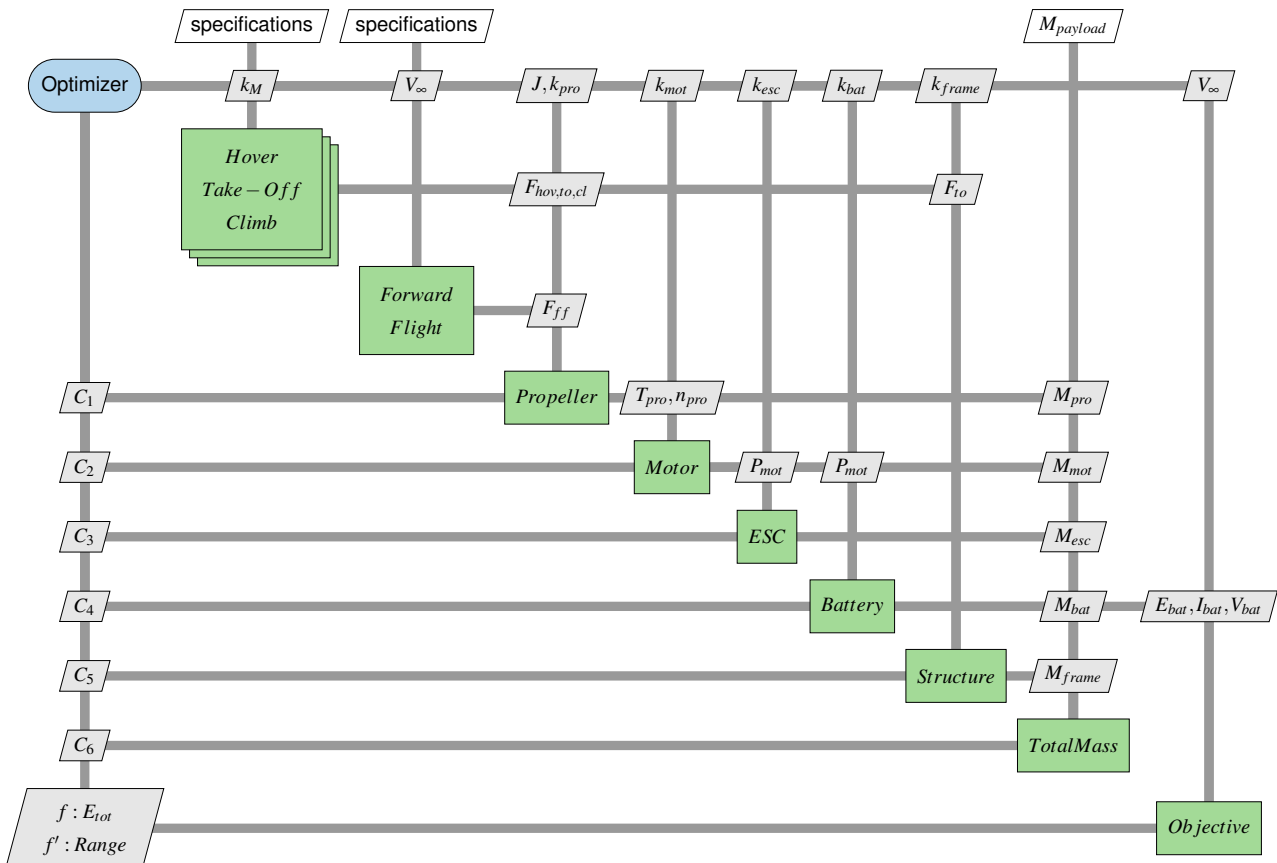
Figure 4 – XDSM diagram for multirotor drone optimization.
