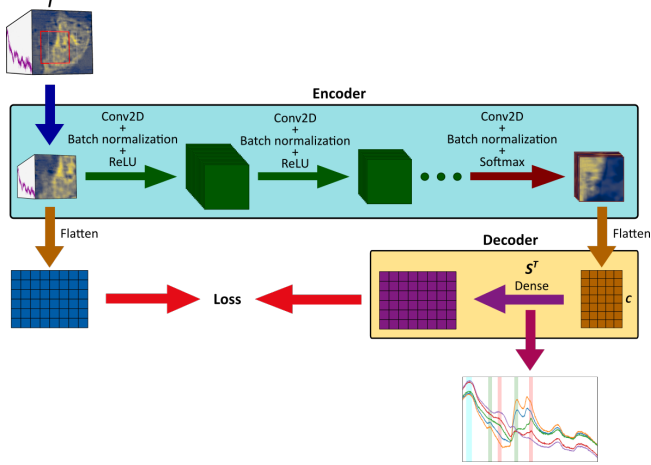
Fig. 1. Our MCR-SSAE process.
