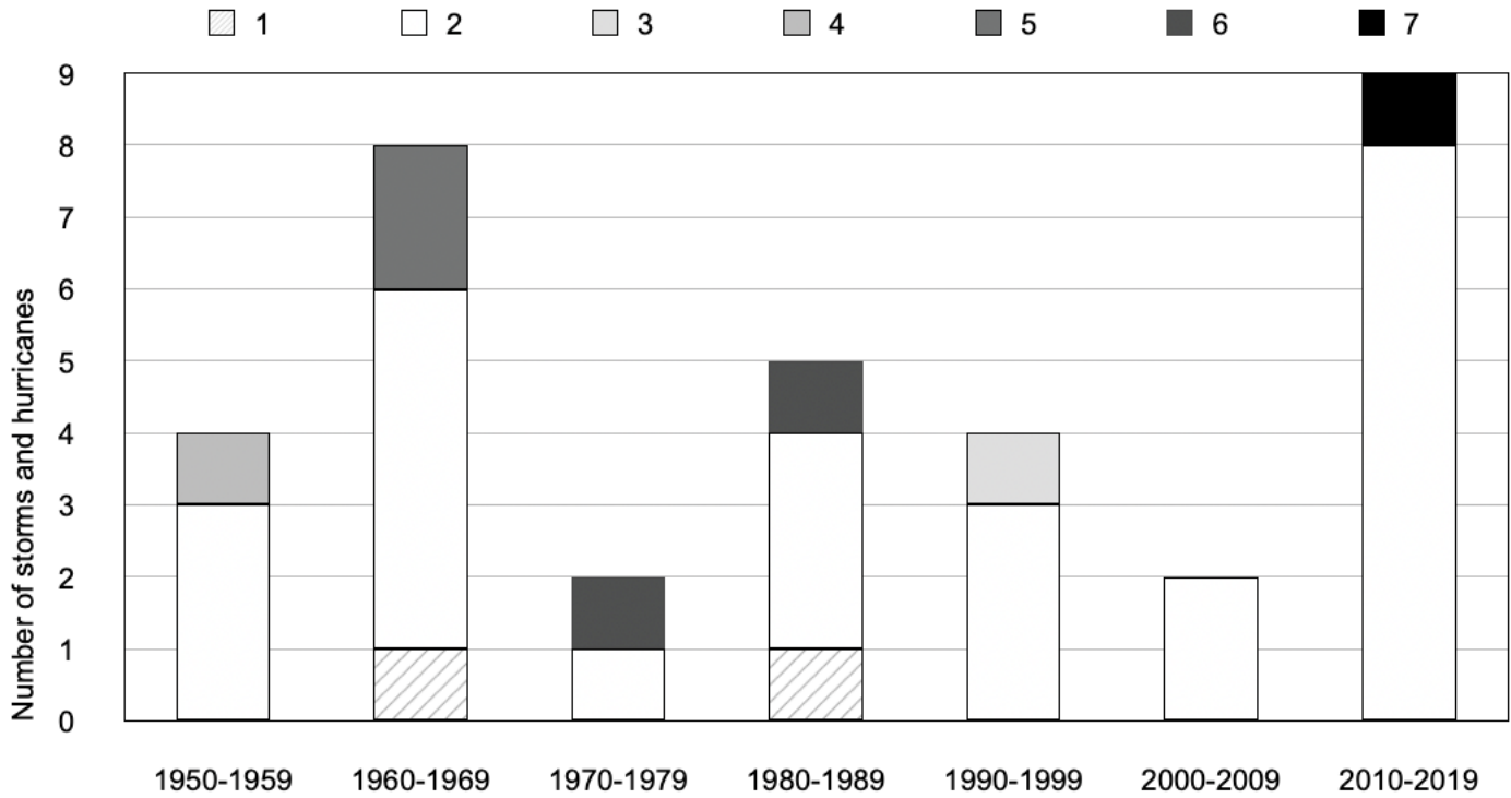
Figure 2 Number and intensity of depressions, tropical storms and hurricanes per decade between 1950 and 2019 with an eye that passed 100 km or less from Dominica. 1. Unnamed storm. 2. Tropical depression or storm (sustained winds of less than 118 km/h). 3. Category 1 hurricane (sustained winds between 119 and 153 km/h). 4. Category 2 hurricane (sustained winds between 154 and 177 km/h). 5. Category 3 hurricane (sustained winds between 178 and 210 km/h). 6. Category 4 hurricane (sustained winds between 211 and 251 km/h). 7. Category 5 hurricane (sustained winds of more than 251 km/h). The class of intensity for each storm depends on the wind speed reached at the point of the trajectory closest to the centroid of the island
