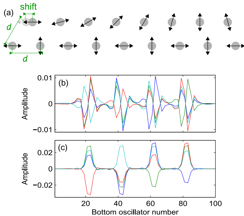
Figure 10. (a) Sketch of a configuration in which the lower row nearest neighbors are not coupled directly, and the top row induces coupling. Only a part of the system, which is made up of 2 \times 100 beads, is drawn here. The angles in the top row are chosen so that an angle of \pi is rotated over 20 beads. This spatial structure is observed in the four longest-lived modes, represented in (b) by showing the amplitude of the mode on the odd-index bottom row beads (blue, green, red, cyan solid lines, from modes 1 to 4, respectively). In the system studied in (b), the top row beads are staggered exactly at the mid point between beads on the bottom row, whereas in (c) the top row beads are shifted by 0.4d from the mid-point. In all cases d = 8 \mu\text{m} , and radius a = 1.74 \mu\text{m} , as in the rest of this work.
