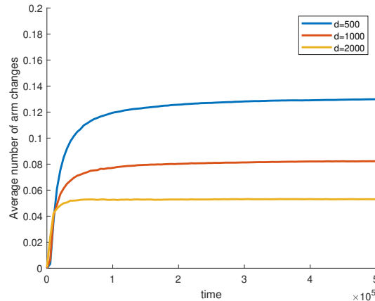
Fig. 5: Average number of arm changes with respect to the number of plays
