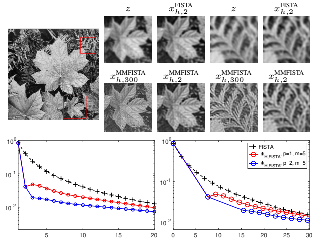
Fig. 1: Top : From left to right : Original 2048 \times 2048 image z , (first row) zoom of the degraded image z for a noise with \sigma = 0.01 and a Gaussian blur of size 40 \times 40 and 7.3 standard deviation and of x_{h,2} computed by FISTA. (second row) zoom of x_{h,2} and x_{h,300} computed by MMFISTA. Bottom: (left) Evolution of F_h versus iterations for MMFISTA with \Phi_{H,FISTA} for p = 1, 2, m = 5 ; (right) Same for CPU time (in sec). \lambda_h = 1.7 \times 10^{-4} .
