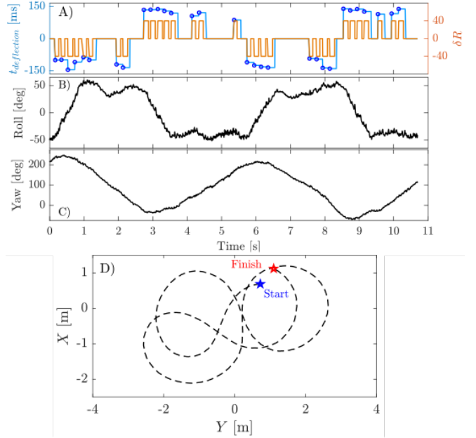
Fig. 5. For closed-loop system identification purpose, a human pilot stabilized the Metafly while a randomized signal was added to the t_{deflection} input (here given by the joystick) in order to enlarge the input frequency range for more accurate system identification. A) For the sake of visualization and for identification purpose, the input t_{deflection} was computed by measuring the time \delta R was hold constant during the identification flight tests. B) Roll. C) Yaw during several banked turns. D) X-Y positions during system identification flight test.
