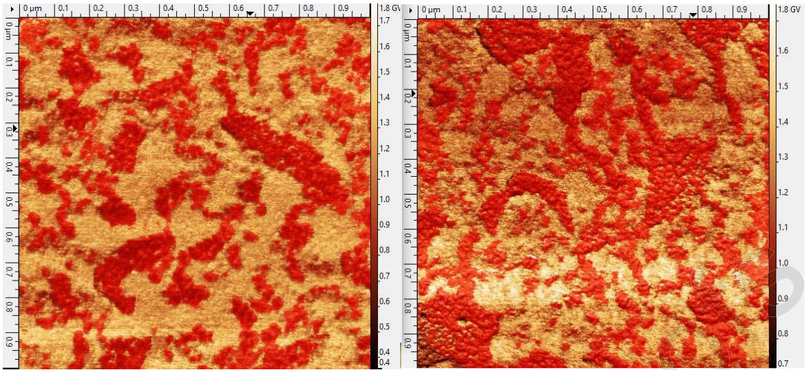
E = 1.16 GPa
