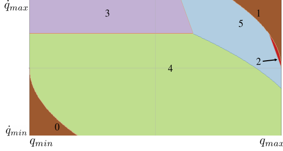
Fig. 2: Feasible state space for q^{\max} = -q^{\min} = 0.5 rad, \dot{q}^{\max} = 2 rad/s, \ddot{q}^{\max} = 10 rad/s 2 , \delta t = 0.1 s, and \bar{w} = \frac{1}{3}\ddot{q}^{\max} . Region 0 represents the unreachable space, while region 1 represents the space that is not viable. In each of the other four regions, a different acceleration upper bound dominates the others. In region 2 it is the one coming from the position inequality (26). In region 3 it is the one coming from the velocity inequality (31). In region 4 it is the acceleration upper bound \ddot{q}^{\max} . In region 5 it is the one coming from the viability inequality (32).
