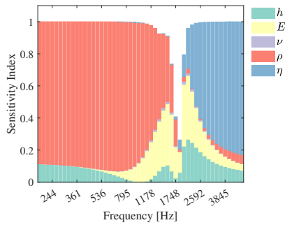
(a) True STL model is used to evaluate the outputs.
