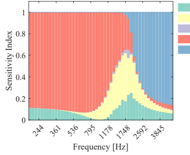
(b) FAST total sensitivity indices.
