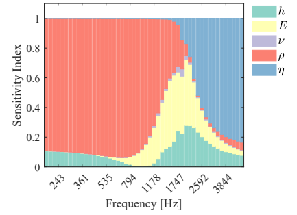
(c) MDI importances.
