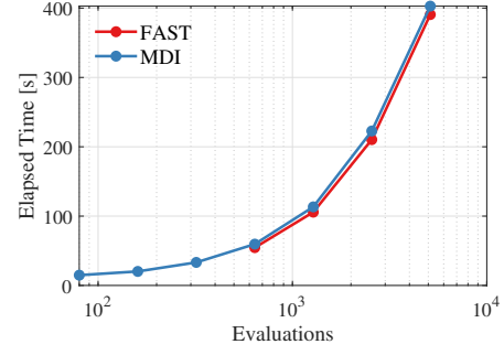
(b) Elapsed time.
