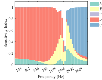
(b) RF-based surrogate is used to predict outputs.
