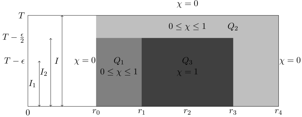
Figure 1: Choice of the cutoff function \chi .
