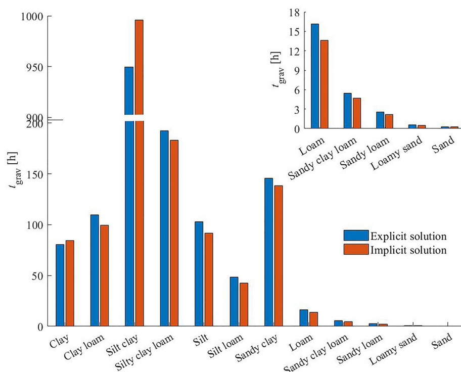
Figure 6. Variations in the soil characteristic time, t_{\text{grav}} , determined using the implicit and explicit solutions (based on three terms) of t_{\text{grav}} for the examined soil textural classes. The inset shows differences between the two approaches for the coarser soils. Note that the ordinate is split for better visualization.
