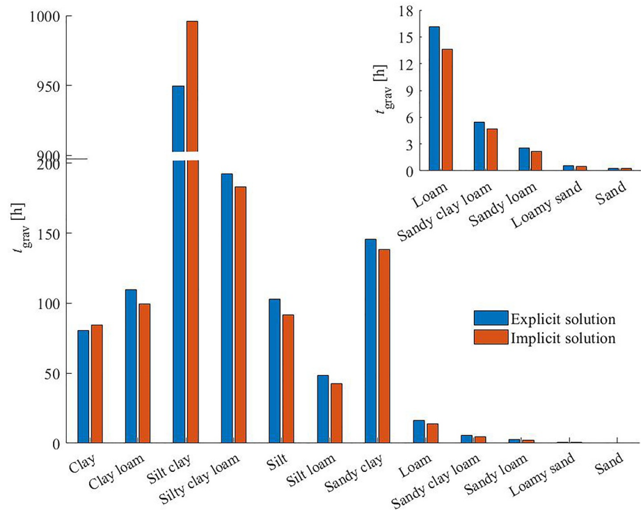
Figure 6. Variations in the soil characteristic time, t_{\text{grav}} , determined using the implicit and explicit solutions (based on three terms) of t_{\text{grav}} for the examined soil textural classes. The inset shows differences between the two approaches for the coarser soils. Note that the ordinate is split for better visualization.
