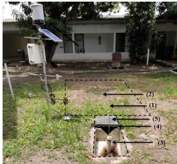
Figure 2. Infiltration trench and monitoring equipment: infiltration trench (1), piezometer (2 and 3), triangular spillway (4), passage box (5) and rain gauge (6).
