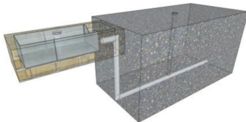
Figure 3. Infiltration trench perspective. (Source: [4]).
