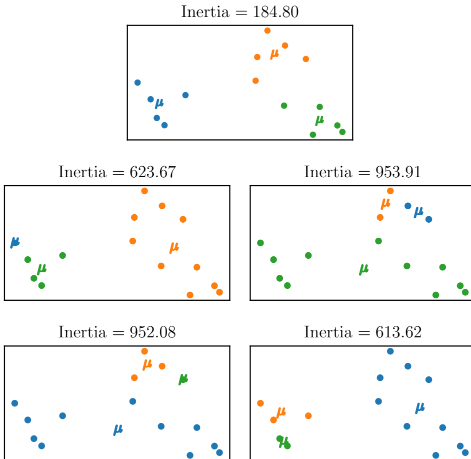
Figure 21: Illustration of the convergence of the k -means algorithm to bad local minima. In the upper figure, the algorithm converged to a global minimum because the inertia is equal to the minimum possible value (184.80), thus the obtained clusters are optimal. In the four other figures, the algorithm converged to a local minima that are not global minima because the inertias are higher than the minimum possible value, thus the obtained clusters are suboptimal.
