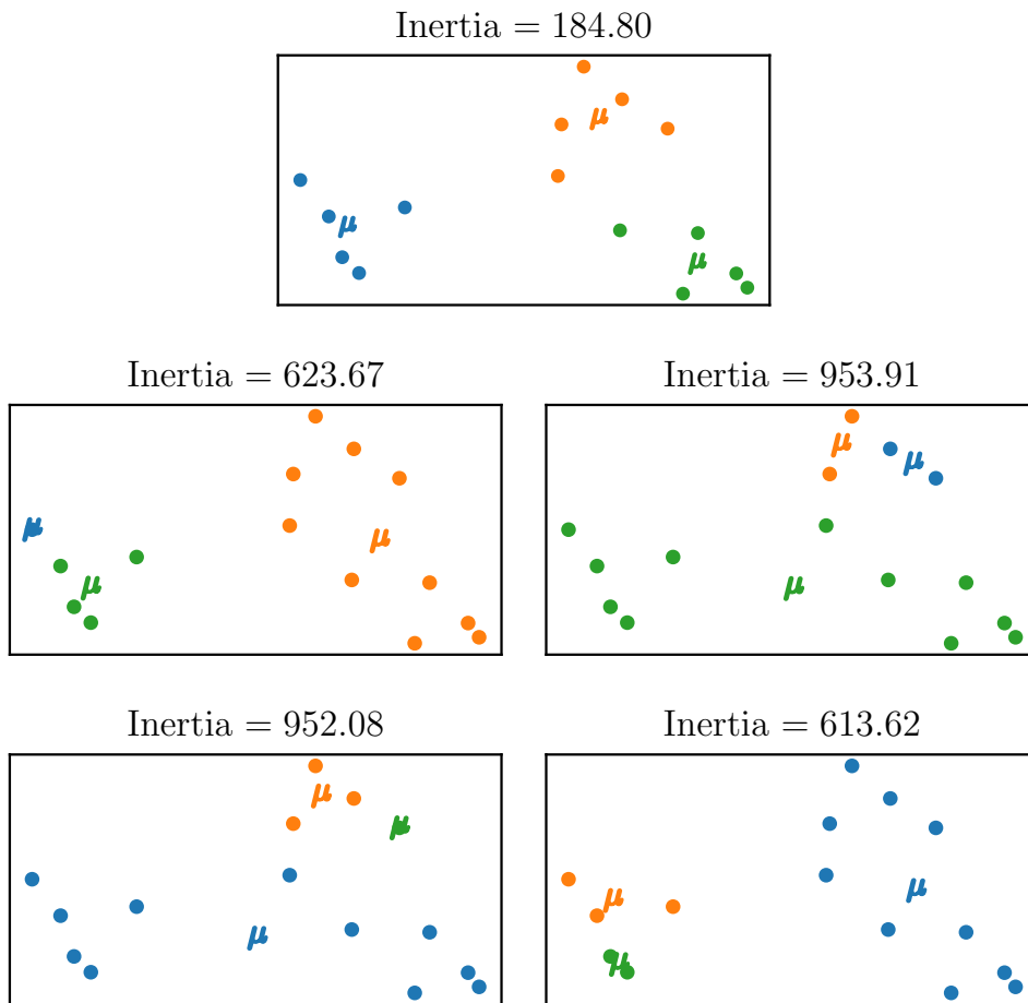
Figure 21: Illustration of the convergence of the k-means algorithm to bad local minima. In the upper figure, the algorithm converged to a global minimum because the inertia is equal to the minimum possible value (184.80), thus the obtained clusters are optimal. In the four other figures, the algorithm converged to a local minima that are not global minima because the inertias are higher than the minimum possible value, thus the obtained clusters are suboptimal.
