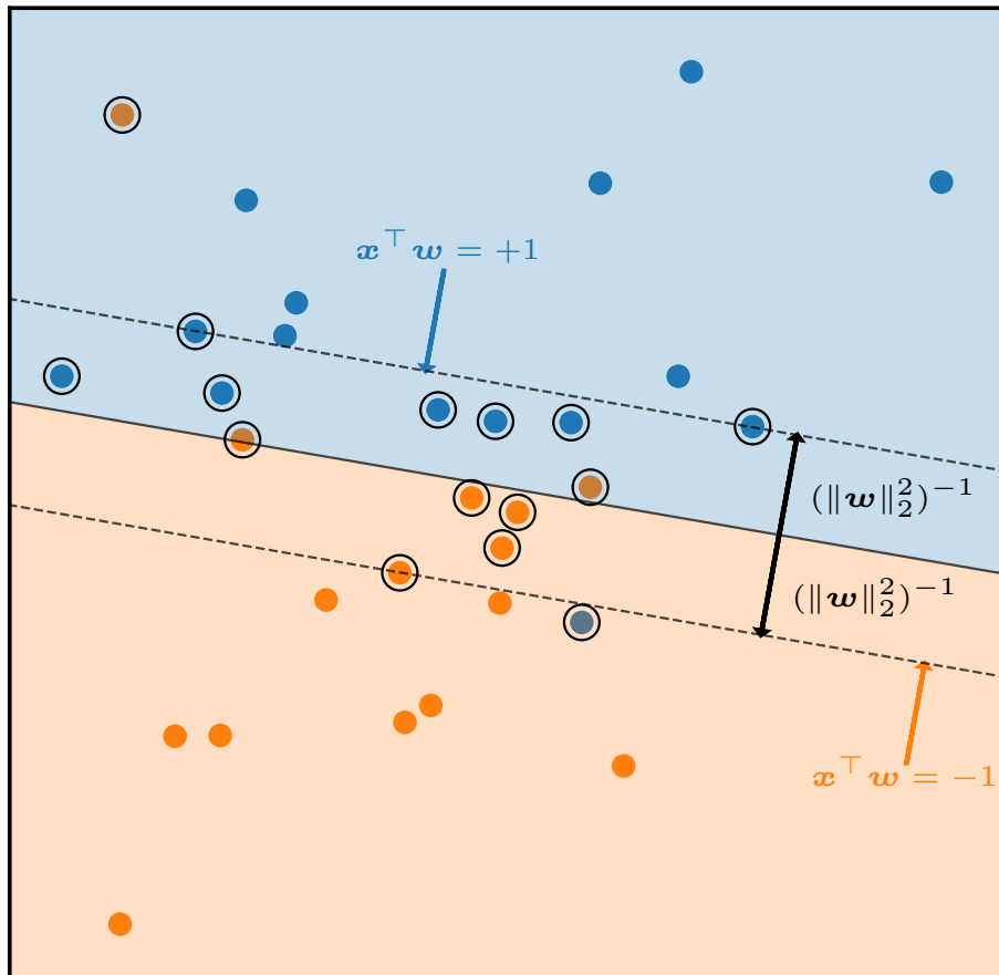
Figure 10: Decision function of a support-vector machine classifier with a linear kernel when both classes are not strictly linearly separable. The support vectors are the training points within the margin of the decision function and the misclassified training points. The support vectors are highlighted with a black circle surrounding them.
