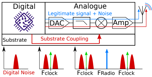
Fig. 1. Screaming channel attacks: Conventional side-channels leak to the RF module in the analog part, present on the same die. This one transmits side-channels at a larger distance (until some meters).
