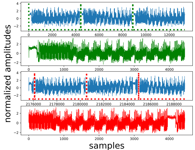
Fig. 3. Segment CPs using the virtual trigger: 1st row: the beginning of the collected trace and the VT positions determined according to the known CP length. 2nd row: a segment aligned to segment start time. 3rd/4th rows: if the length is not precise enough, a drift appears in start times, and hence VT indicates a very different point in CPs at the end of the trace.
