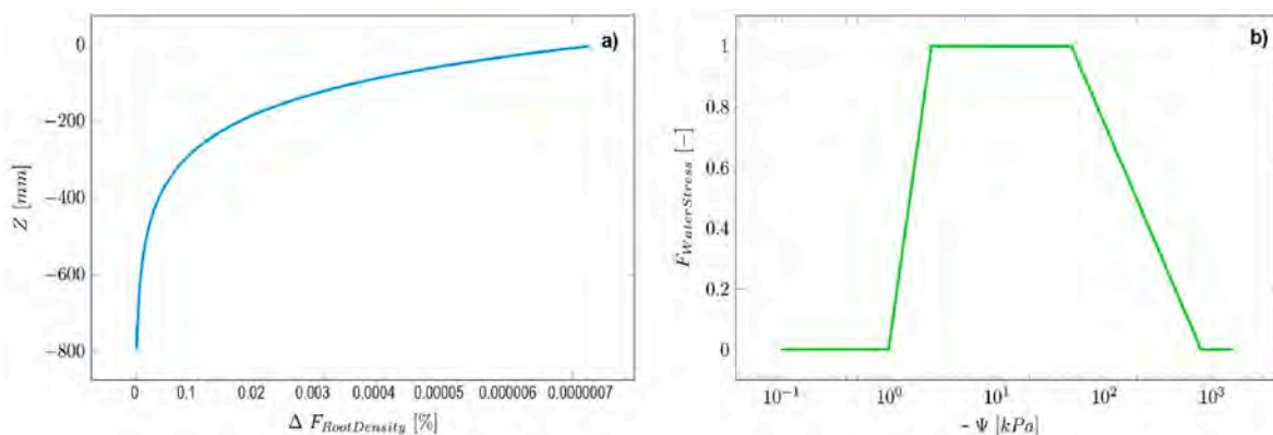
Fig. 5. Pasture grass models used for all field sites: (a) root density function plotted with depth and (b) schematic of the Feddes et al. (1978) plant water stress function.
