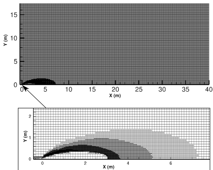
Figure 5: DSMC simulation mesh using a eight levels refinement adaptation method according to the value of the numerical Knudsen number K_{n,num} = \lambda/\Delta x , where \lambda is the particles mean free path, and \Delta x the cell size
