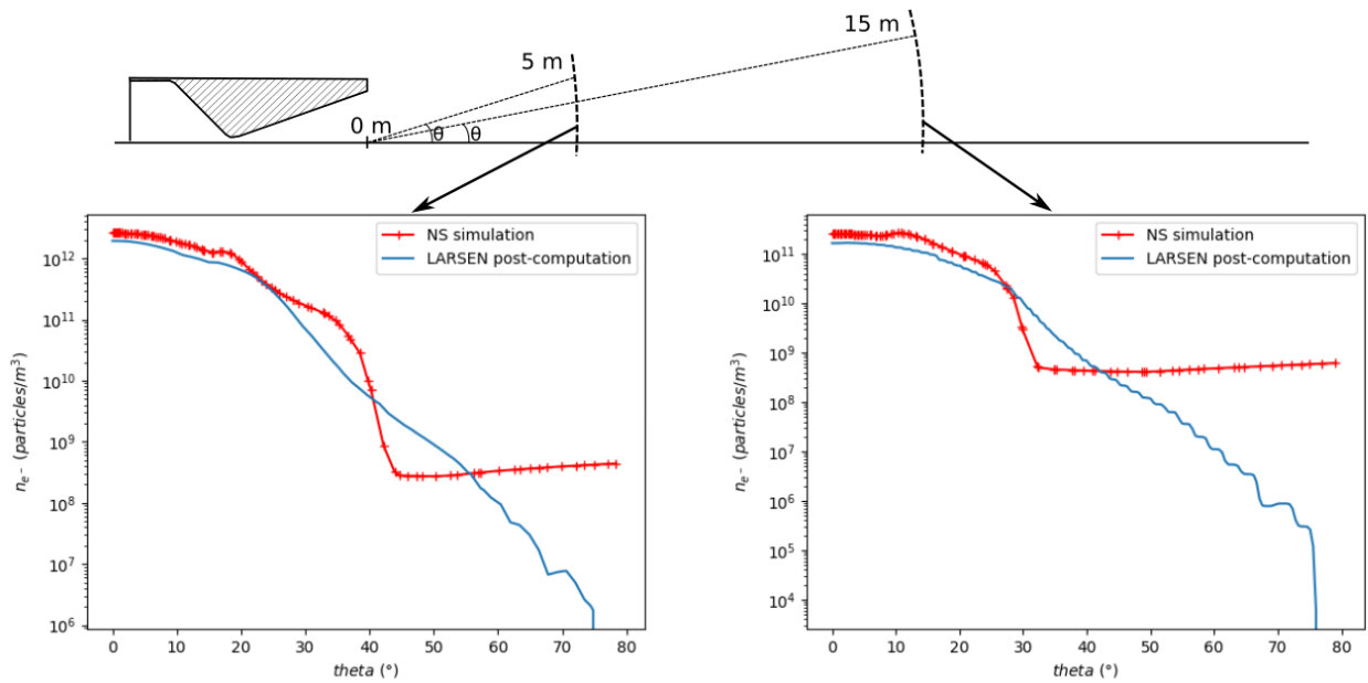
Figure 10: Angular profiles of the electron density n_{e^-} obtained with the simple NS simulation and with the hybrid methodology (LARSEN post-computation) along a 5\text{ m} radius circle (left) and a 15\text{ m} radius circle (right) around the nozzle
