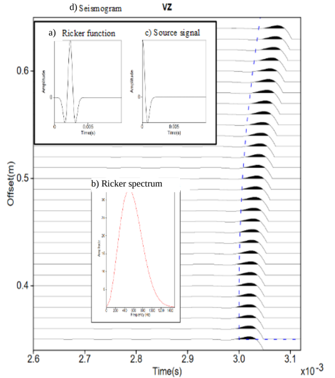
Figure 3 : Simulation results with finite differences in the case of homogeneous medium; a) Ricker function; b) Ricker function spectrum; c) Source signal used in finite difference simulations; d) The vertical velocity wavefield recovered at the receivers. The estimated arrival times computed by using the method presented in section 3 are plotted dashed curve
