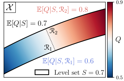
Figure 2: Intuition. In the feature space \mathcal{X} , the level set of confidence S = 0.7 displays \mathbb{E}[Q | S] = 0.7 , which we expect from a calibrated classifier. However, a partition of the level set into 2 regions \mathcal{R}_1 and \mathcal{R}_2 reveals that \mathbb{E}[Q | S, \mathcal{R}_1] = 0.6 while \mathbb{E}[Q | S, \mathcal{R}_2] = 0.8 , suggesting a high grouping loss. Intra-region variances \mathbb{V}_h[Q | S, \mathcal{R}_1] and \mathbb{V}_h[Q | S, \mathcal{R}_2] remain uncaptured.
