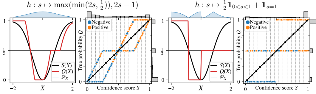
Figure 10: Calibrated and optimal accuracy. Example of calibrated classifiers S constructed from links h following the procedure described in Appendix B.1. The accuracy of these two classifiers is optimal as Q and S are on the same side of the decision threshold ( \frac{1}{2} ) wherever Q \neq \frac{1}{2} . However, confidence scores S are almost everywhere different from the true posterior probabilities Q . Calibration curves (in black on 2 nd and 4 th plot) are obtained from 1 million samples.
