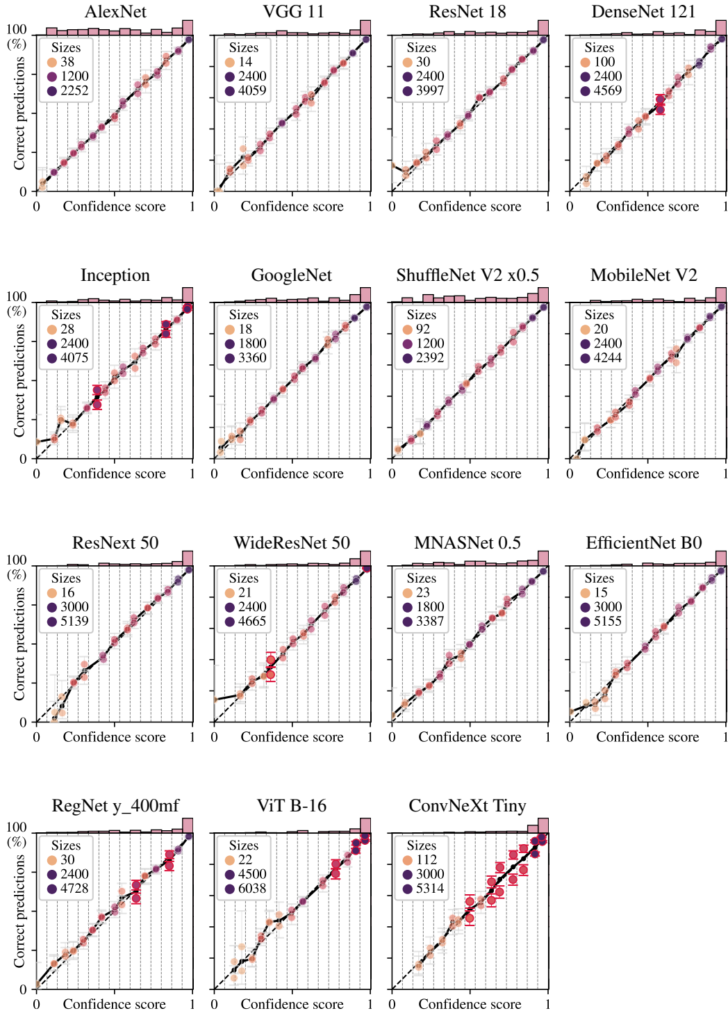
Figure 26: Vision : Fraction of correct predictions versus confidence score of predicted class ( \max_k S_k ) on ImageNet-1K (validation set) for small versions of pre-trained networks, with isotonic recalibration. In each bin on confidence scores, the level set is partitioned into 2 regions with a decision stump constrained to one balanced split, with a 50-50 train-test split strategy.
