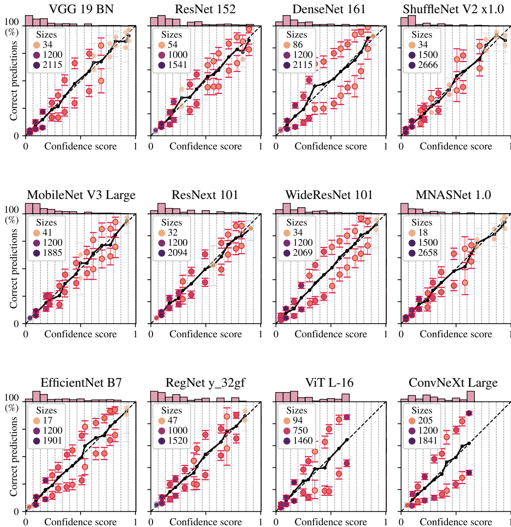
Figure 19: Vision: Fraction of correct predictions versus confidence score of predicted class ( \max_k S_k ) on ImageNet-R for best versions of pre-trained networks, with isotonic recalibration. In each bin on confidence scores, the level set is partitioned into 2 regions with a decision stump constrained to one balanced split, with a 50-50 train-test split strategy.
