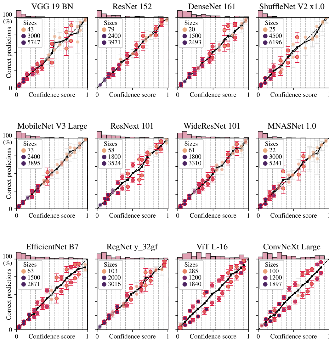
Figure 23: Vision: Fraction of correct predictions versus confidence score of predicted class ( \max_k S_k ) on ImageNet-C for best versions of pre-trained networks, with isotonic recalibration. In each bin on confidence scores, the level set is partitioned into 2 regions with a decision stump constrained to one balanced split, with a 50-50 train-test split strategy.
