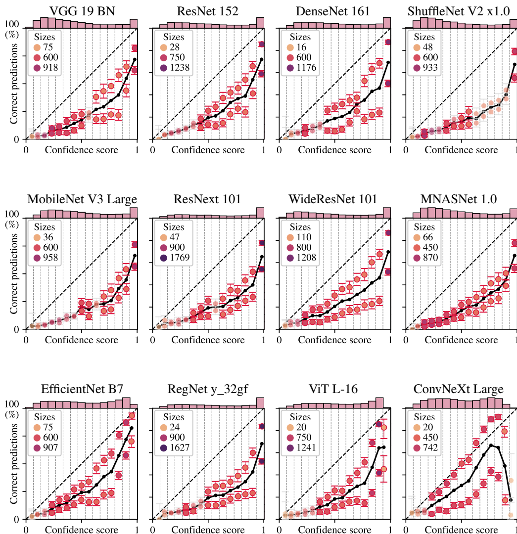
Figure 17: Vision: Fraction of correct predictions versus confidence score of predicted class ( \max_k S_k ) on ImageNet-R for best versions of pre-trained networks, without post-hoc recalibration. In each bin on confidence scores, the level set is partitioned into 2 regions with a decision stump constrained to one balanced split, with a 50-50 train-test split strategy.
