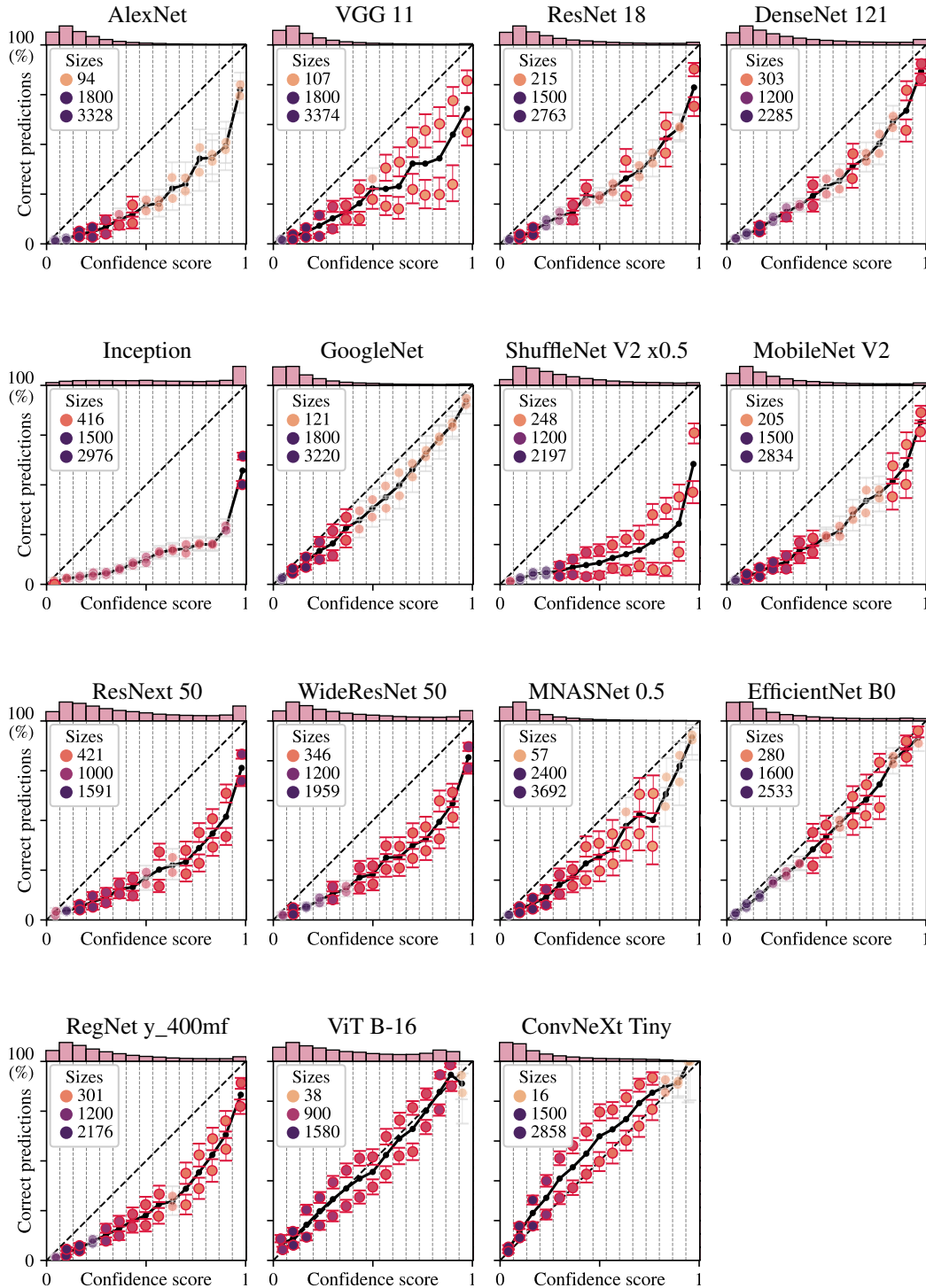
Figure 20: Vision : Fraction of correct predictions versus confidence score of predicted class ( \max_k S_k ) on ImageNet-C for small versions of pre-trained networks, without post-hoc recalibration. In each bin on confidence scores, the level set is partitioned into 2 regions with a decision stump constrained to one balanced split, with a 50-50 train-test split strategy.
