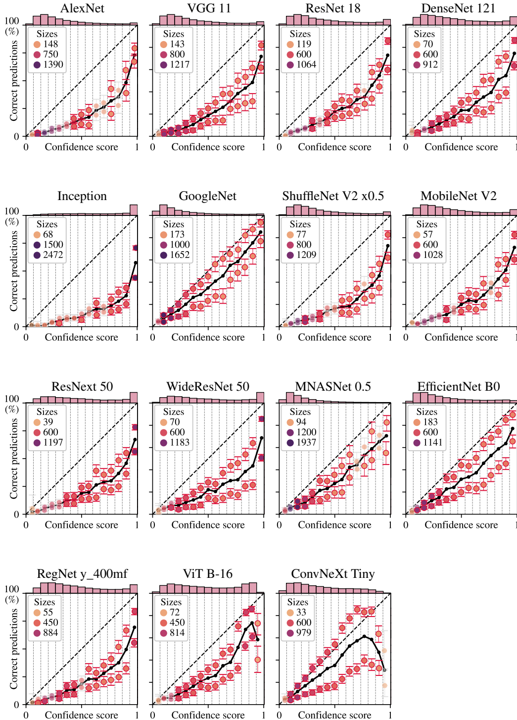
Figure 15: Vision : Fraction of correct predictions versus confidence score of predicted class ( \max_k S_k ) on ImageNet-R for small versions of pre-trained networks, without post-hoc recalibration. In each bin on confidence scores, the level set is partitioned into 2 regions with a decision stump constrained to one balanced split, with a 50-50 train-test split strategy.
