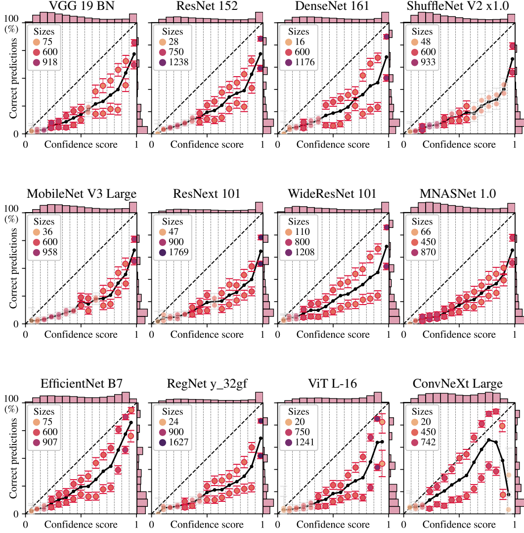
Figure 17: Vision : Fraction of correct predictions versus confidence score of predicted class ( \max_k S_k ) on ImageNet-R for best versions of pre-trained networks, without post-hoc recalibration. In each bin on confidence scores, the level set is partitioned into 2 regions with a decision stump constrained to one balanced split, with a 50-50 train-test split strategy.
