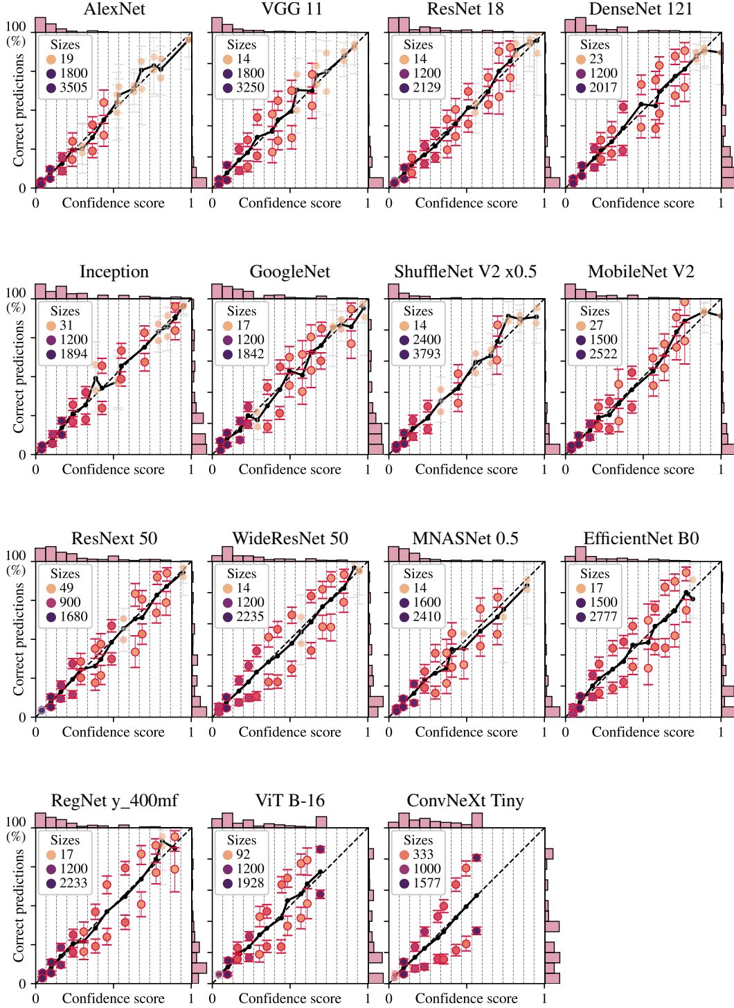
Figure 18: Vision: Fraction of correct predictions versus confidence score of predicted class (max k S k ) on ImageNet-R for small versions of pre-trained networks, with isotonic recalibration. In each bin on confidence scores, the level set is partitioned into 2 regions with a decision stump constrained to one balanced split, with a 50-50 train-test split strategy.
