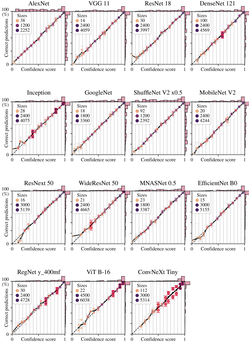
Figure 26: Vision : Fraction of correct predictions versus confidence score of predicted class ( \max_k S_k ) on ImageNet-1K (validation set) for small versions of pre-trained networks, with isotonic recalibration. In each bin on confidence scores, the level set is partitioned into 2 regions with a decision stump constrained to one balanced split, with a 50-50 train-test split strategy.
