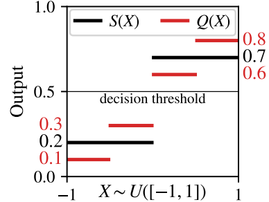
Figure 1: A calibrated binary classifier with optimal accuracy and confidence scores S(X) everywhere different from the true posterior probabilities Q(X) .
