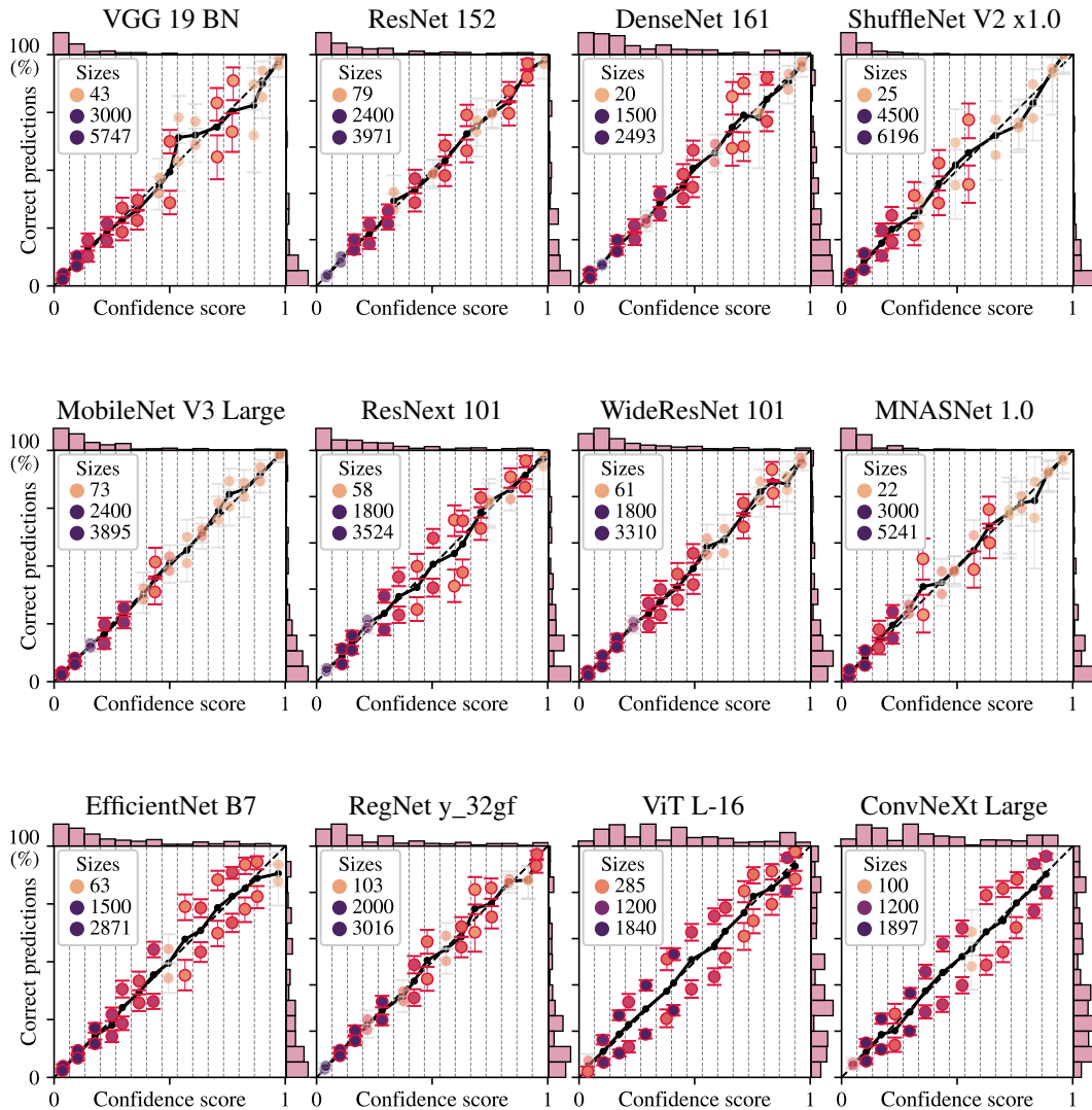
Figure 23: Vision : Fraction of correct predictions versus confidence score of predicted class ( \max_k S_k ) on ImageNet-C for best versions of pre-trained networks, with isotonic recalibration. In each bin on confidence scores, the level set is partitioned into 2 regions with a decision stump constrained to one balanced split, with a 50-50 train-test split strategy.
