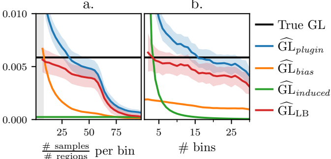
Figure 4: Simulation: estimating the grouping loss lower bound \widehat{GL}_{LB} on a simulated problem ( Appendix B.2 , Figure 11 ). Right has a fixed ratio \frac{\# \text{ samples}}{\# \text{ regions}} = 30 per bin. Bins are equal-width. Averaged curves are plotted with a \pm 1 standard deviation envelop.
