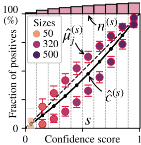
Figure 5: Grouping diagram. Calibration curve of a binned binary classifier augmented with the estimated region scores \hat{\mu}_j for a partitioning of each level set into 2 regions. Region sample sizes are plotted as a gradient color. The classifier is binned into 10 equal-width bins whose sample sizes n^{(s)} are given as an histogram. A Clopper-Pearson 95% confidence interval is plotted on the region scores. Regions for which the calibrated score \hat{c}^{(s)} lie within this interval are grayed out.
